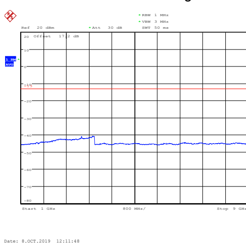
LTE Band 5 1.4MHz CH-High 1GHz~9GHz
