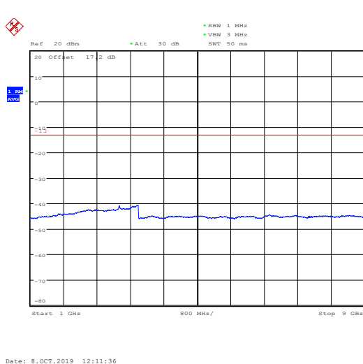
LTE Band 5 1.4MHz CH-Middle 1GHz~9GHz
