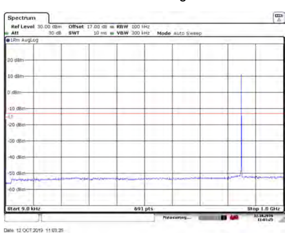
LTE Band 5 1.4MHz CH-High 9kHz~1GHz
