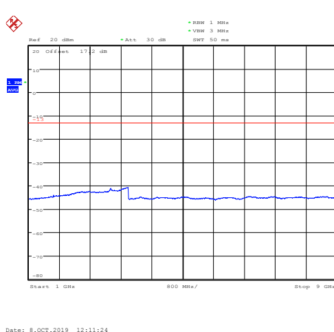
LTE Band 5 1.4MHz CH-Low 1GHz~9GHz
