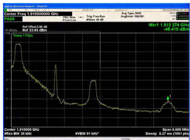
LTE Band 2 3MHz 64QAM 1RB CH-High
