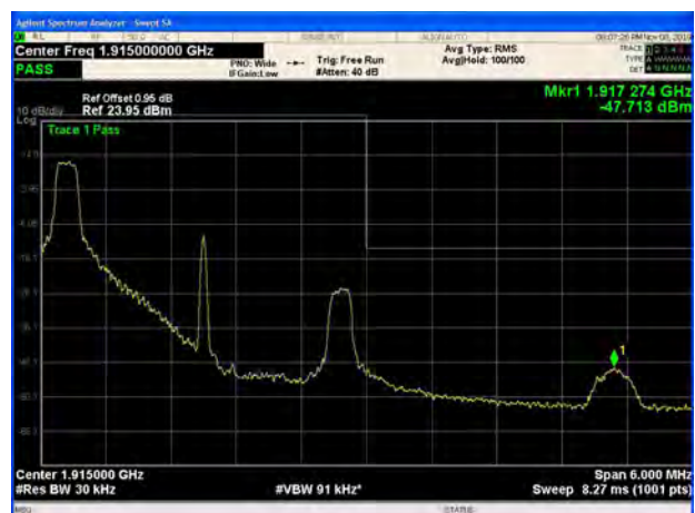
LTE Band 25 3MHz 64QAM 1RB CH-High
