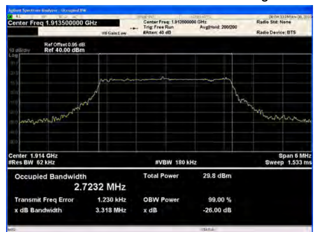
LTE Band 25 3MHz 64QAM CH-High
