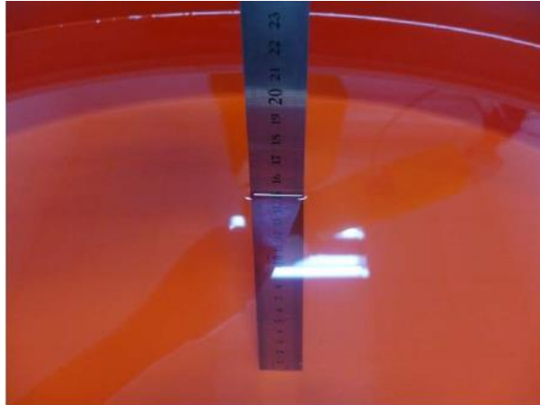
Photo 1: Tissue Simulant Liquid for Head 2600
