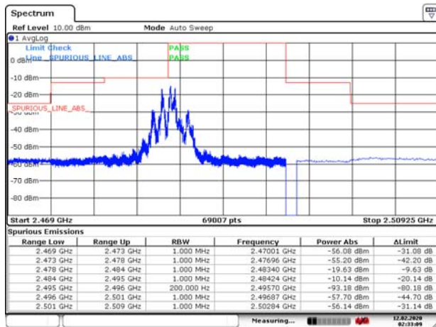
LTE Band 53 1.4MHz QPSK 100%RB CH-Low
