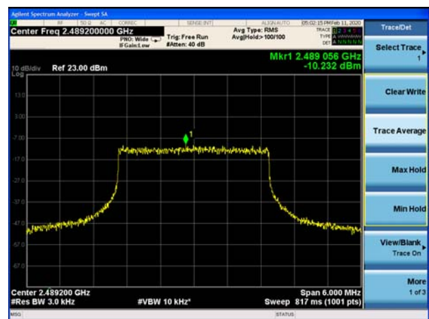
LTE Band 53 3MHz QPSK 1RB CH-High
