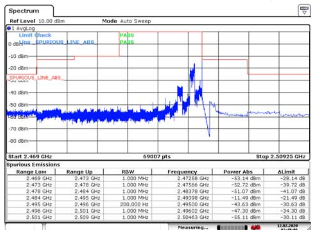
LTE Band 53 3MHz QPSK 1RB CH-High
