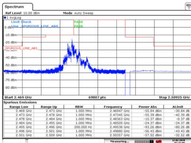
LTE Band 53 3MHz QPSK 1RB CH-Low
