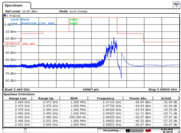
LTE Band 53 1.4MHz QPSK 100%RB CH-High
