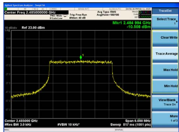
LTE Band 53 3MHz QPSK 1RB CH-Middle
