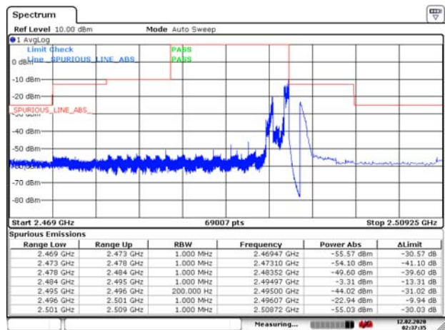
LTE Band 53 1.4MHz QPSK 1RB CH-High
