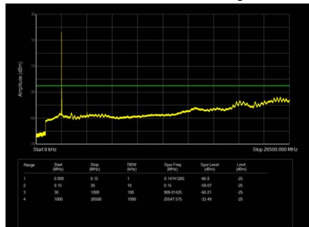
LTE Band 41 20MHz CH-High
