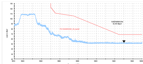
802.11n HT20-Channel 165: Peak
