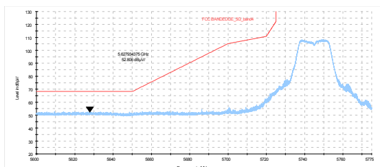
802.11n HT40-Channel 151: Peak
