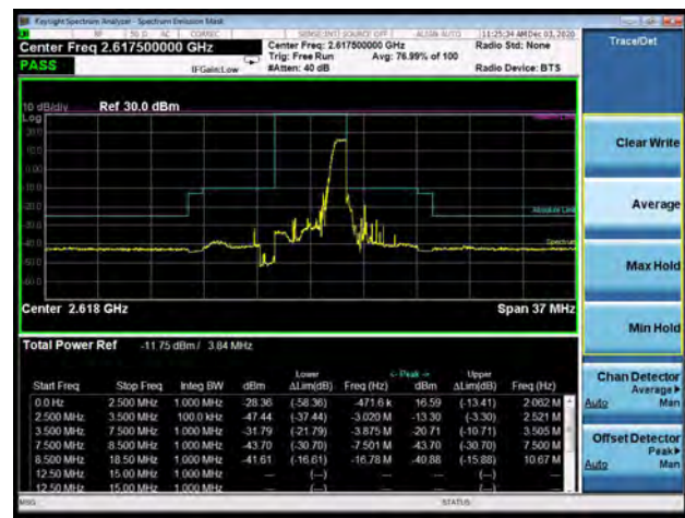
LTE Band 38 QPSK 5MHz CH-High, 100%RB
