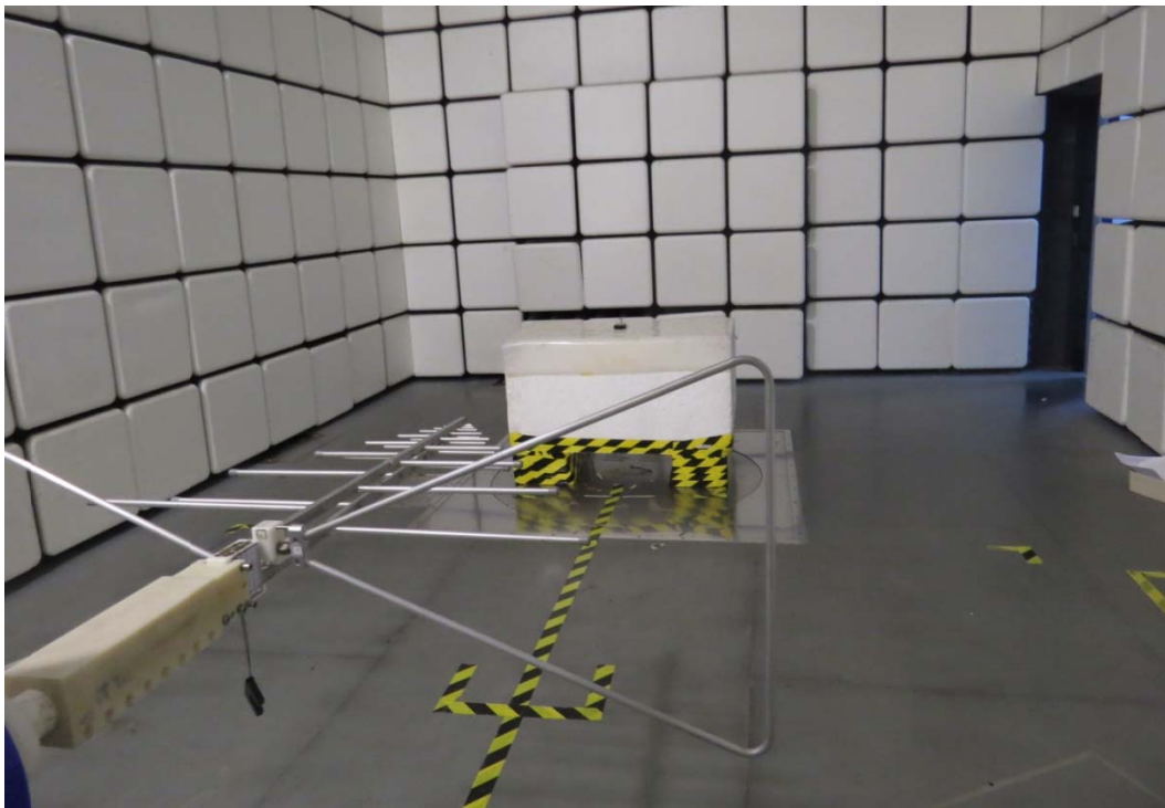
30MHz-1GHz
