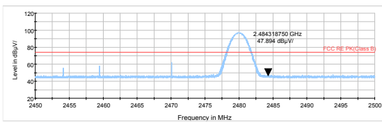
3DH5-Channel 78: Peak
