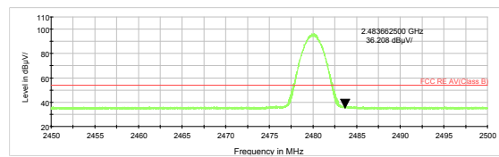
3DH5-Channel 78: Average
