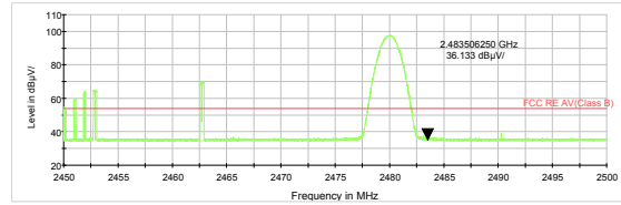
DH5-Channel 78: Average
