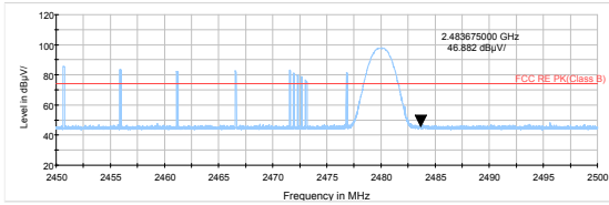
DH5-Channel 78: Peak
