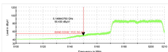
802.11n HT40-Channel 38: Average
