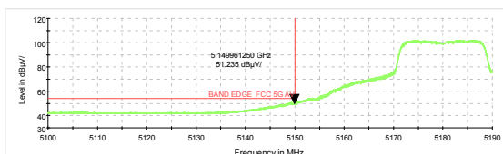
802.11n HT20-Channel 36: Peak
