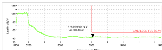
802.11n HT20-Channel 48: Peak
