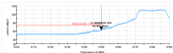
802.11a-Channel 36: Average
