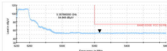
802.11a-Channel 48: Average
