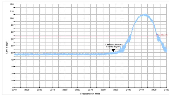
802.11b-Channel 1 Peak
