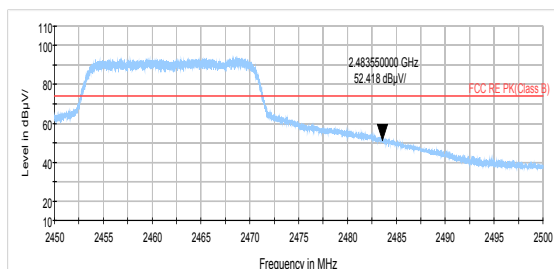
802.11g-Channel 11 Peak
