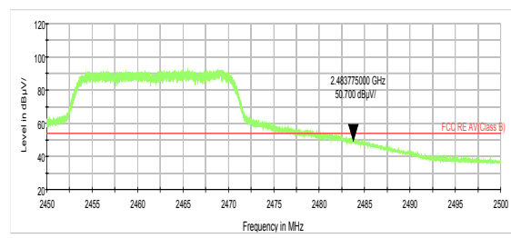
802.11g-Channel 11 Average
