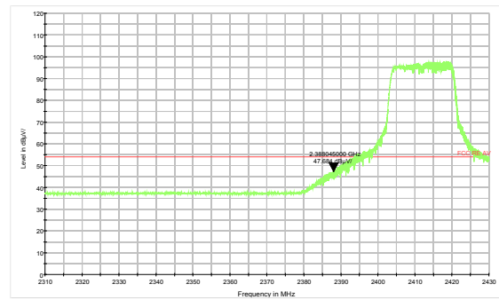
802.11g-Channel 1 Average
