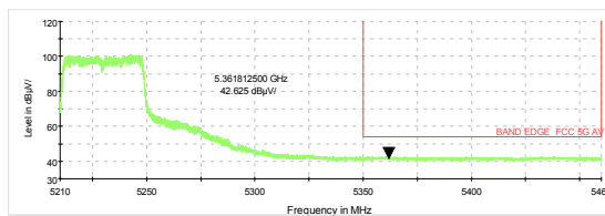
802.11ac VHT80- Channel 42: Average
