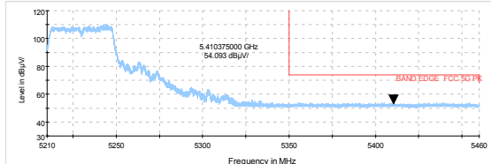
802.11n HT40-Channel 46: Peak
