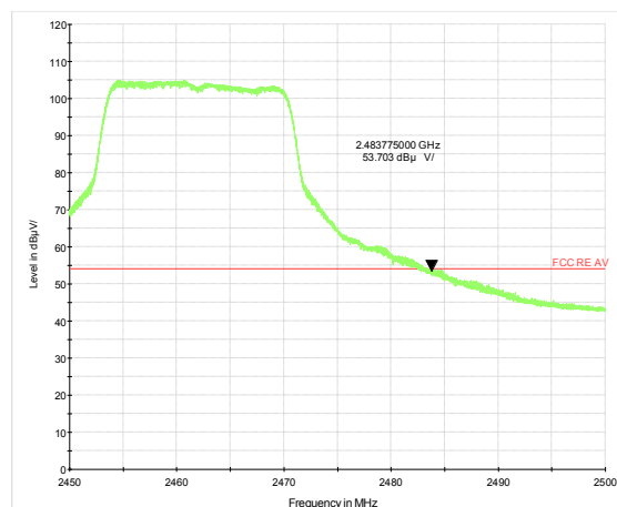
802.11g-Channel 11 Average
