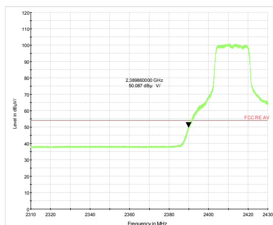
802.11g-Channel 1 Average
