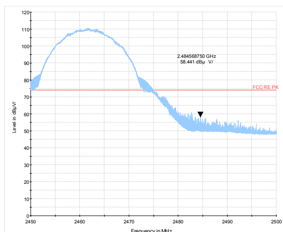
802.11b-Channel 11 Peak
