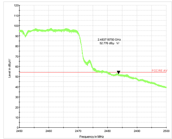
802.11n HT40 -Channel 9 Average
