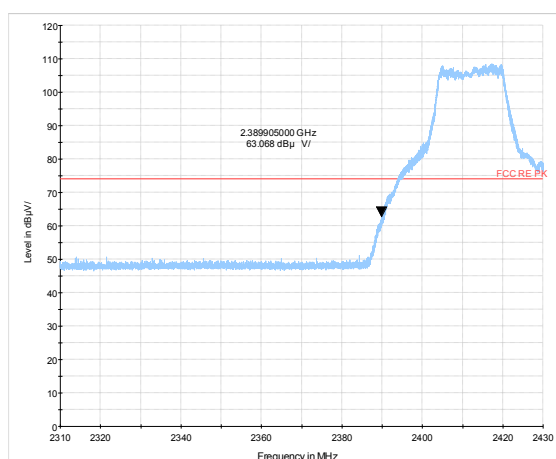
802.11g-Channel 1 Peak
