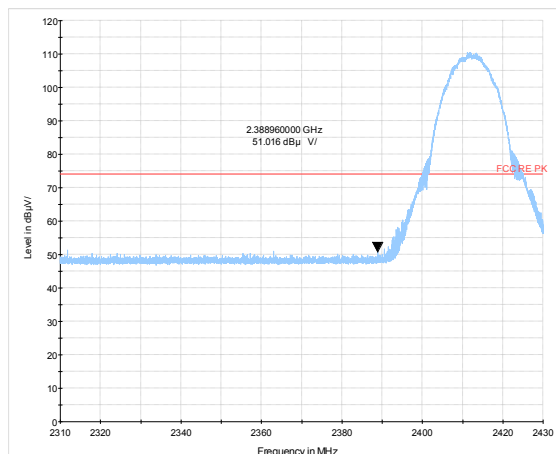
802.11b-Channel 1 Peak
