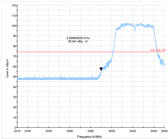
802.11n HT40 -Channel 3 Peak
