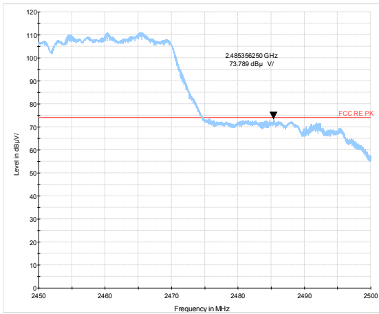
802.11n HT40 -Channel 9 Peak
