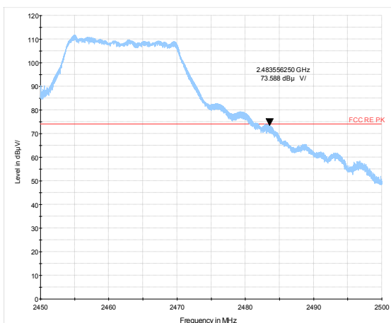
802.11g-Channel 11 Peak
