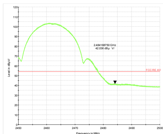
802.11b-Channel 11 Average
