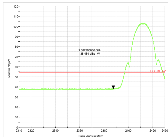
802.11b-Channel 1 Average
