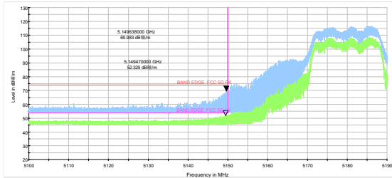
802.11n HT20 -Channel 36: Peak & Average
