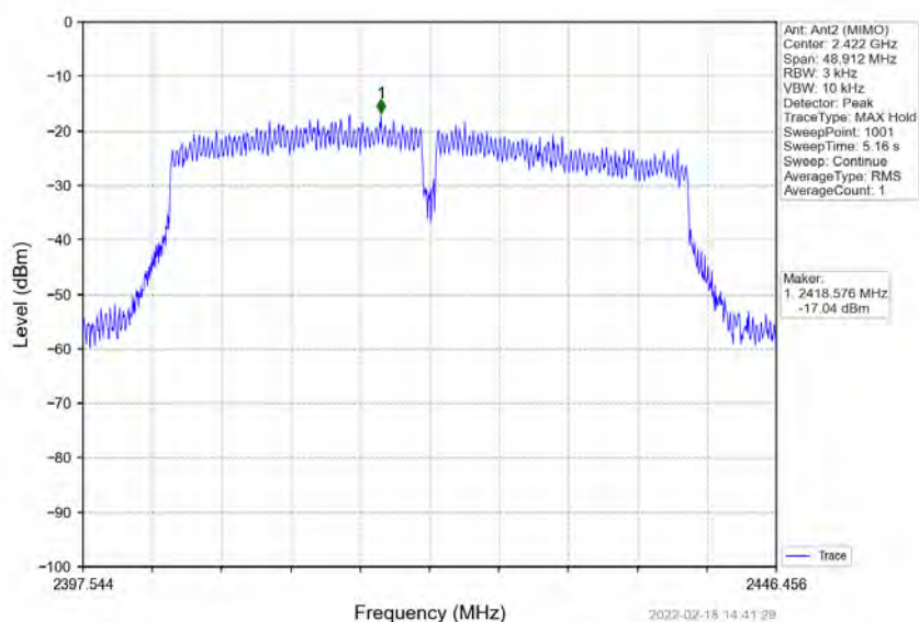
802.11n(HT40)_LCH_2422MHz_MIMO NTN
