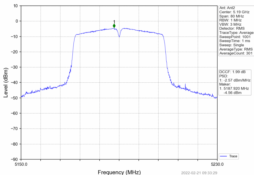
802.11ac(VHT40)_LCH_5190MHz_MIMO_NTNV
