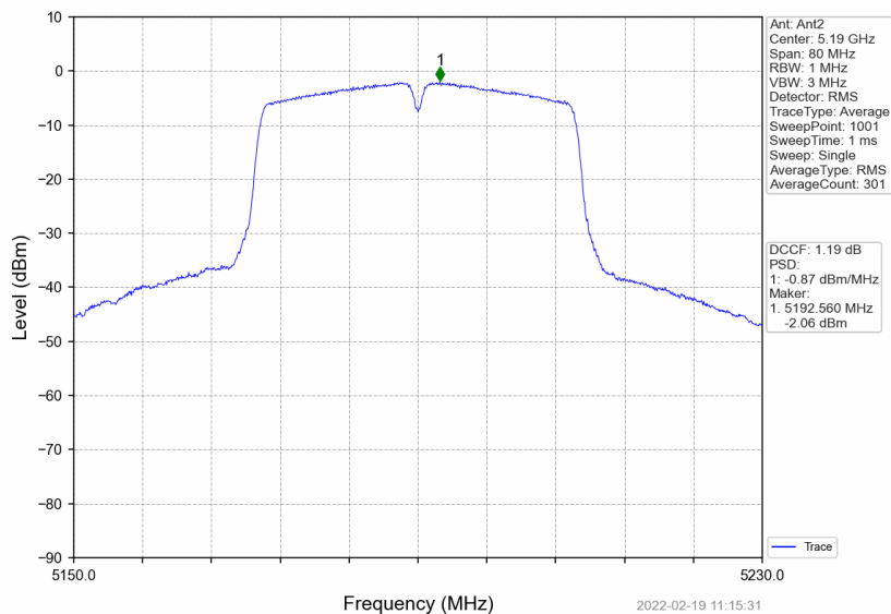
802.11n(HT40)_LCH_5190MHz_MIMO_NTNV
