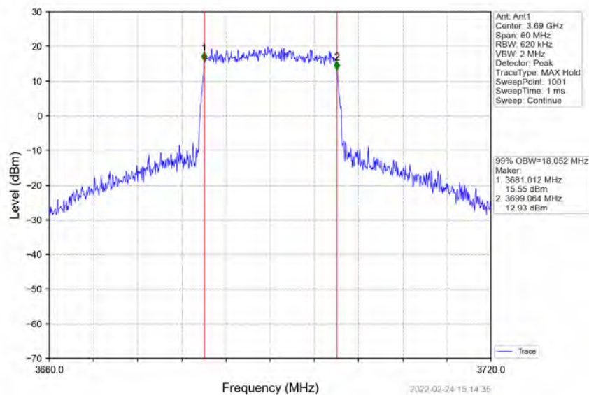
Band48_20MHz_64QAM_HCH_3690MHz_RB_100_0_NTNV
