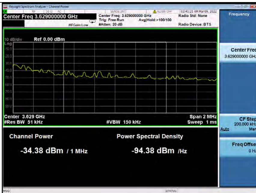
Band48_5MHz_64QAM MCH_3625MHz_RB_25_0_NTNV
