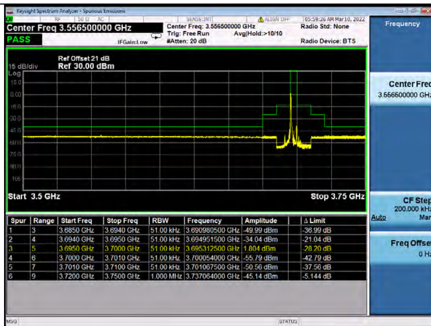
Band48_5MHz_64QAM_HCH_3697.5MHz_RB_1_24_NTNV (Integrated Power for 3693-3694MHz)
