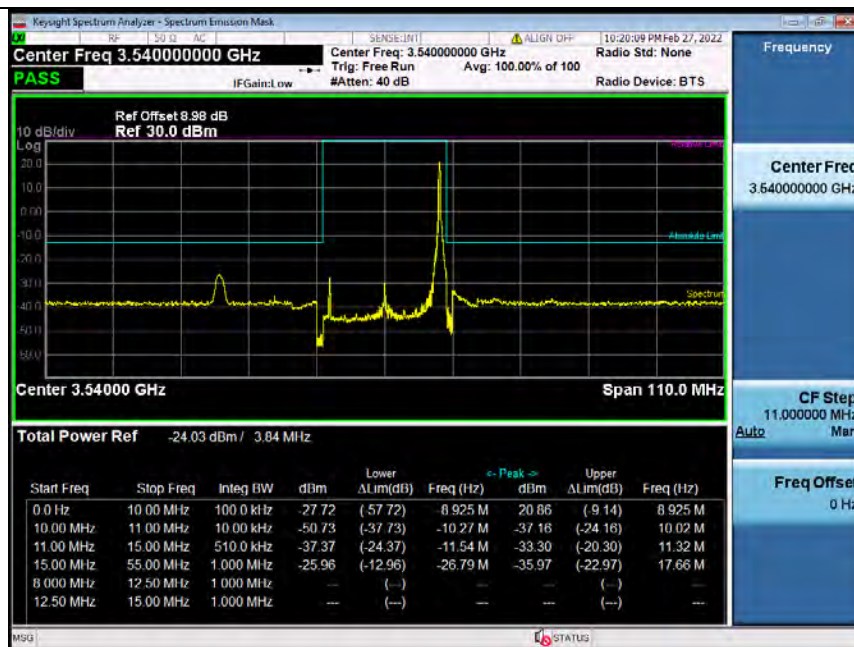
Band42H_20MHz_16QAM_HCH_3540MHz_RB_100_0_NTNV_Bandedge
