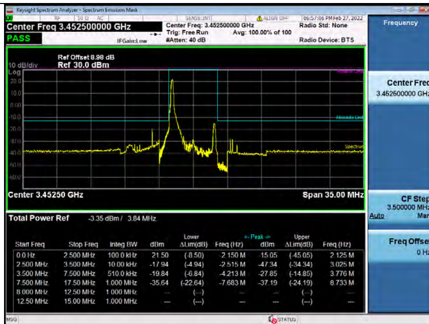
Band42H_5MHz_QPSK_LCH_3452.5MHz_RB_25_0_NTNV_Bandedge
