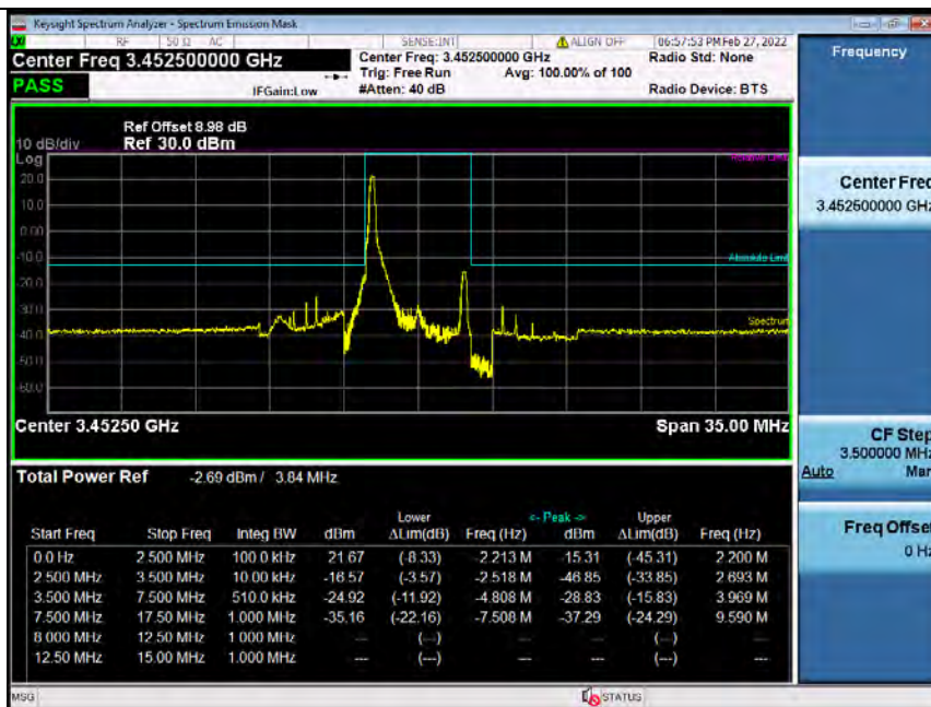
Band42H_5MHz_64QAM_LCH_3452.5MHz_RB_25_0_NTNV_Bandedge
