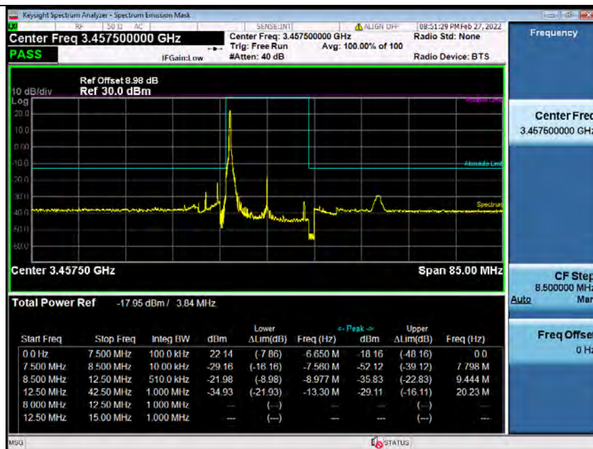
Band42H_15MHz_64QAM_LCH_3457.5MHz_RB_75_0_NTNV_Bandedge
