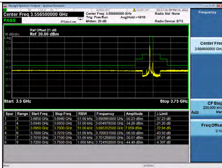
Band48_5MHz_QPSK_HCH_3697.5MHz_RB_1_0_NTNV (Integrated Power for 3693-3694MHz)
