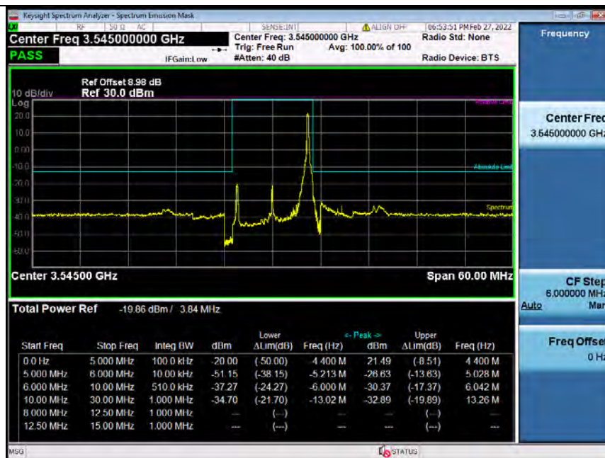
Band42H_10MHz_16QAM_HCH_3545MHz_RB_50_0_NTNV_Bandedge
