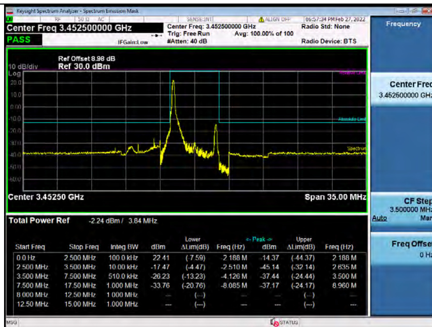
Band42H_5MHz_16QAM_LCH_3452.5MHz_RB_25_0_NTNV_Bandedge
