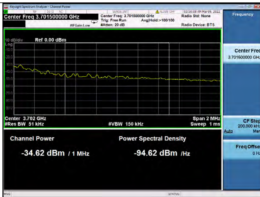
Band48_5MHz_64QAM_HCH_3697.5MHz_RB_25_0_NTNV
