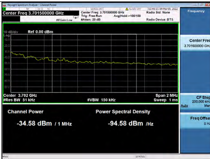
Band48_5MHz_QPSK_HCH_3697.5MHz_RB_25_0_NTNV
