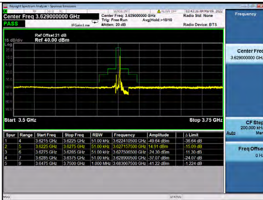
Band48_5MHz_QPSK_MCH_3625MHz_RB_1_24_NTNV (Integrated Power for 3628.5-3629.5MHz)
