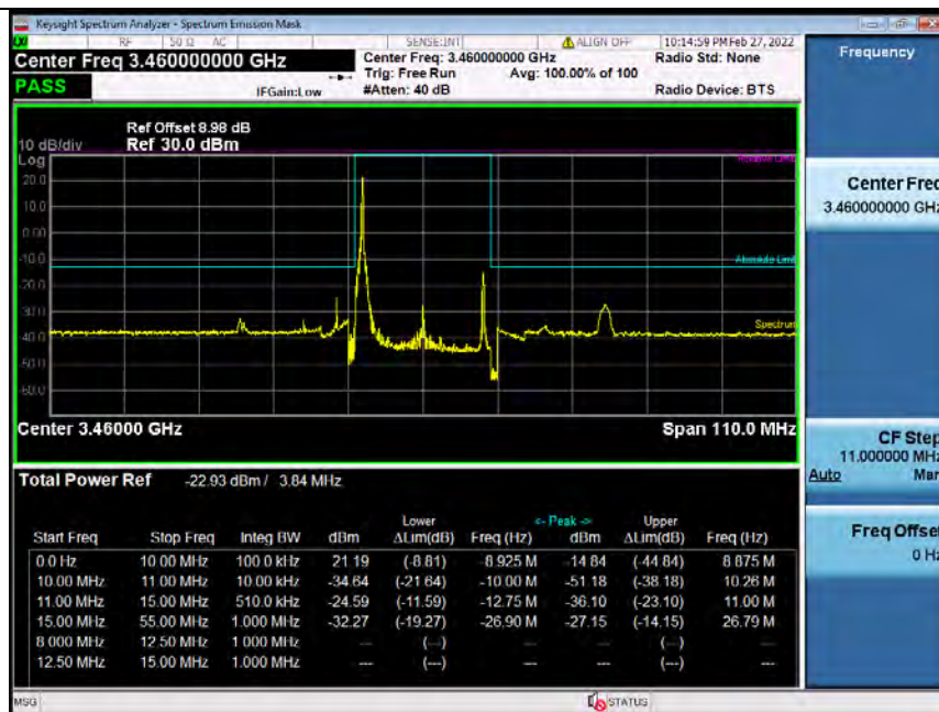
Band42H_20MHz_16QAM_LCH_3460MHz_RB_100_0_NTNV_Bandedge
