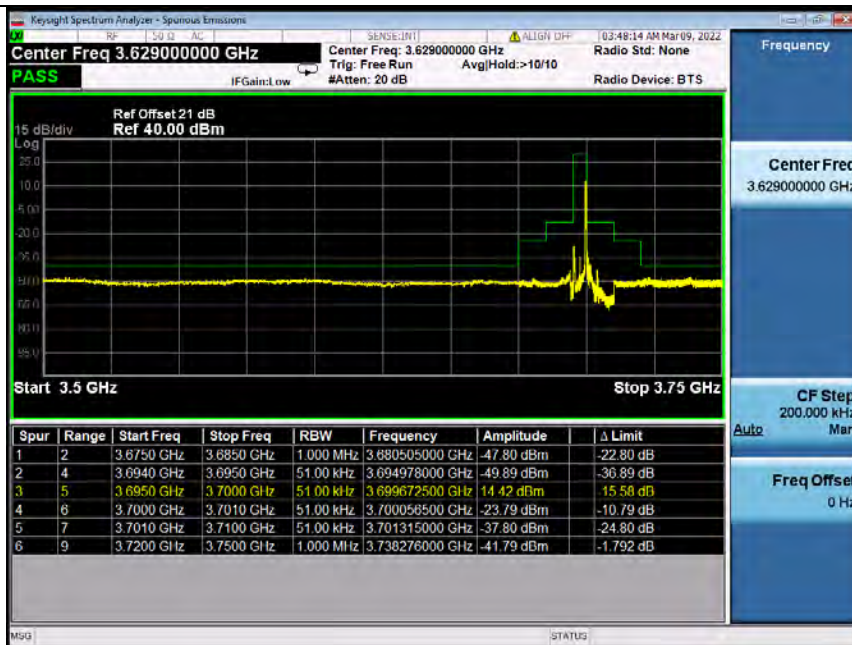
Band48_5MHz_16QAM_HCH_3697.5MHz_RB_1_24_NTNV (Integrated Power for 3701-3702MHz)
