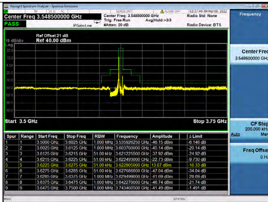
Band48_5MHz_64QAM_MCH_3625MHz_RB_1_0_NTNV (Integrated Power for 3620.5-3621.5MHz)
