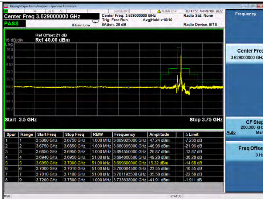
Band48_5MHz_64QAM_HCH_3697.5MHz_RB_1_24_NTNV (Integrated Power for 3701-3702MHz)
