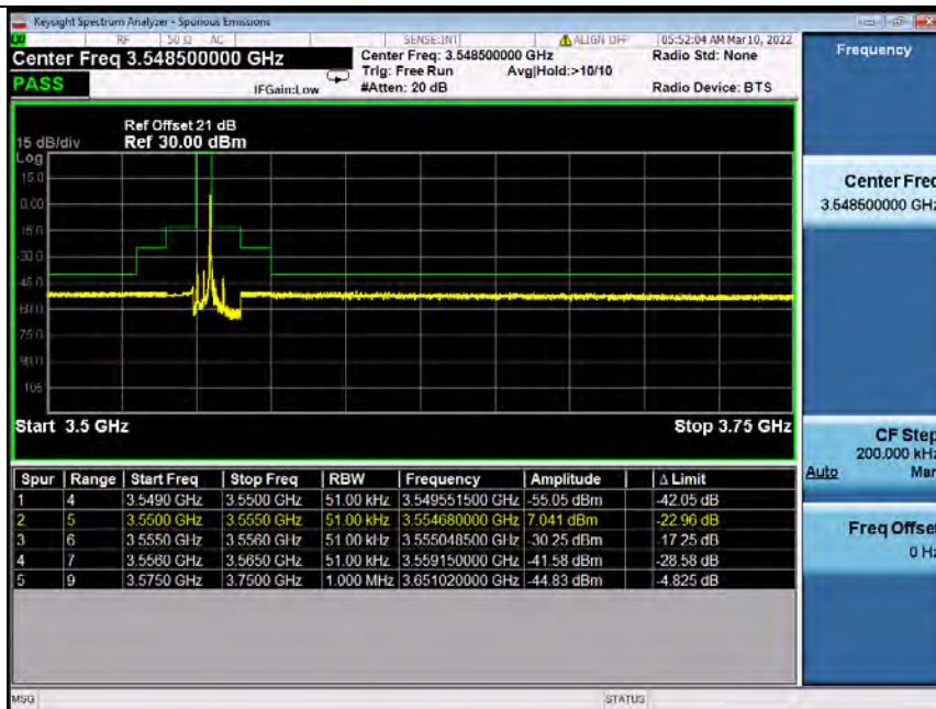
Band48_5MHz_16QAM_LCH_3552.5MHz_RB_1_24_NTNV (Integrated Power for 3556-3557MHz)
