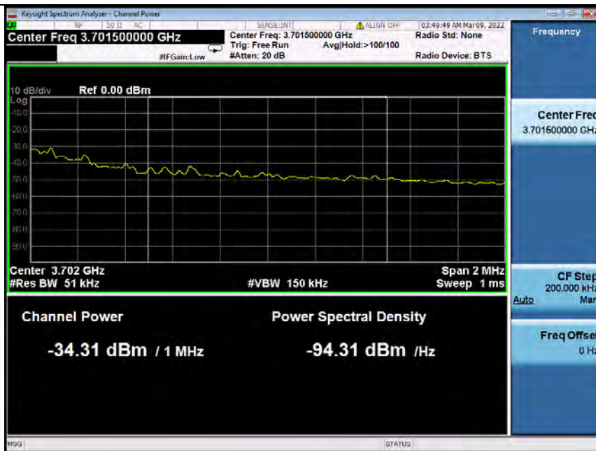
Band48_5MHz_16QAM_HCH_3697.5MHz_RB_25_0_NTNV
