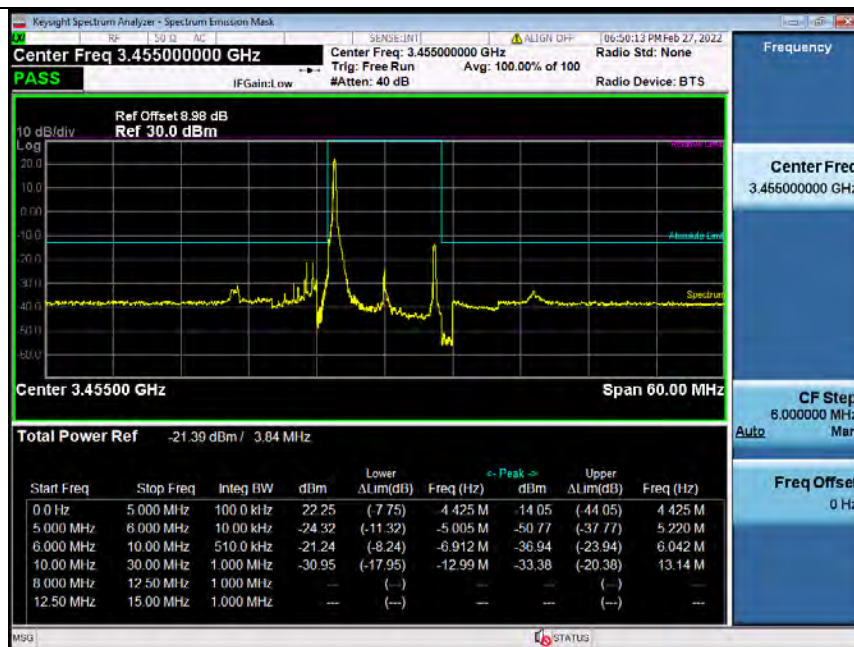
Band42H_10MHz_16QAM_LCH_3455MHz_RB_50_0_NTNV_Bandedge
