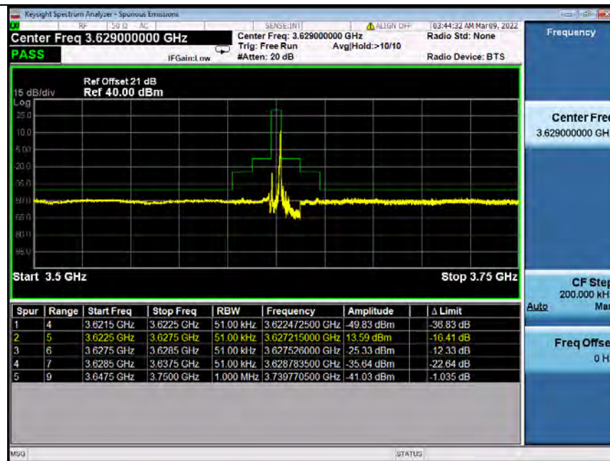
Band48_5MHz_64QAM_MCH_3625MHz_RB_1_24_NTNV (Integrated Power for 3628.5-3629.5MHz)
