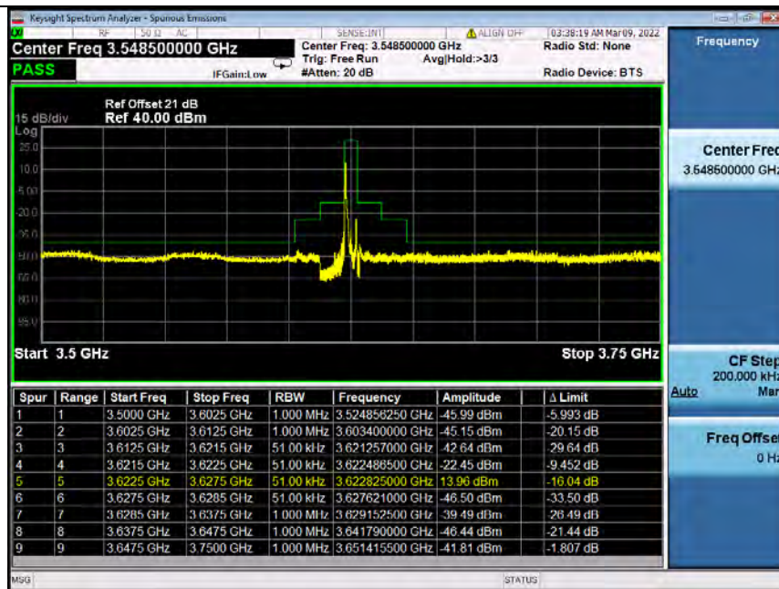
Band48_5MHz_16QAM_MCH_3625MHz_RB_1_0_NTNV (Integrated Power for 3620.5-3621.5MHz)
