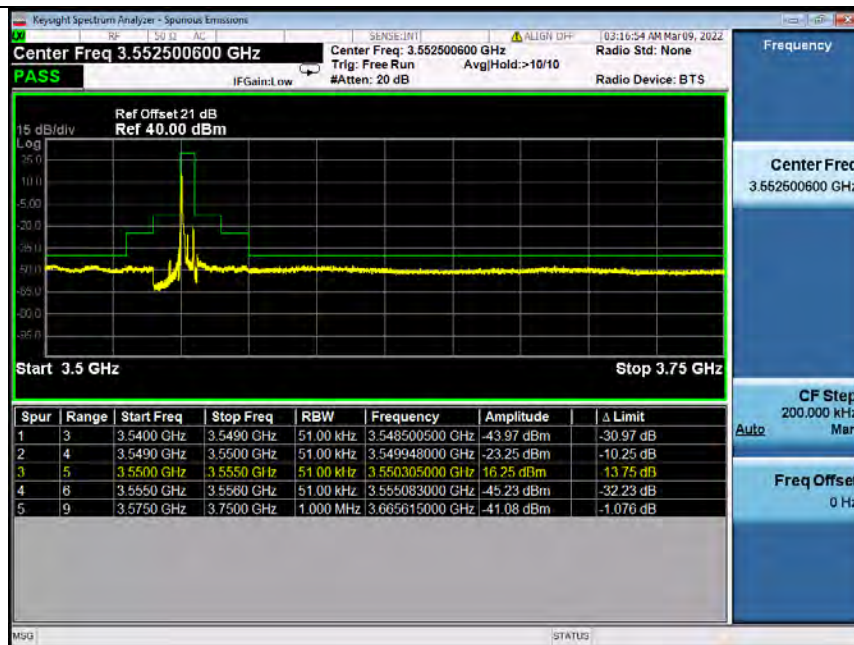
Band48_5MHz_QPSK_LCH_3552.5MHz_RB_1_0_NTNV (Integrated Power for 3548-3549MHz)
