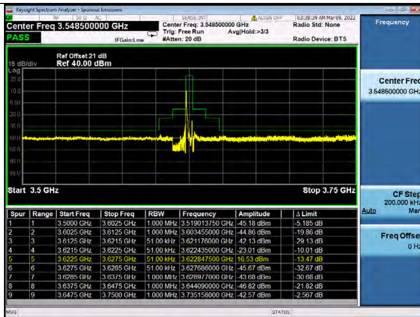
Band48_5MHz_QPSK_MCH_3625MHz_RB_1_0_NTNV (Integrated Power for 3620.5-3621.5MHz)
