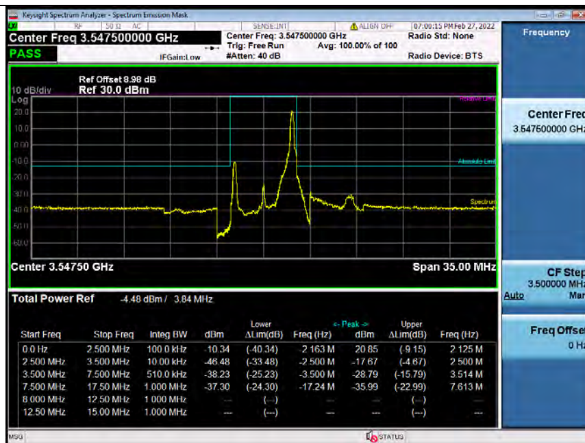
Band42H_5MHz_64QAM_HCH_3547.5MHz_RB_25_0_NTNV_Bandedge
