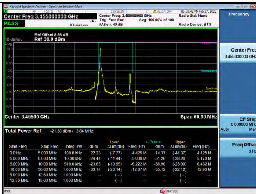
Band42H_10MHz_64QAM_LCH_3455MHz_RB_50_0_NTNV_Bandedge
