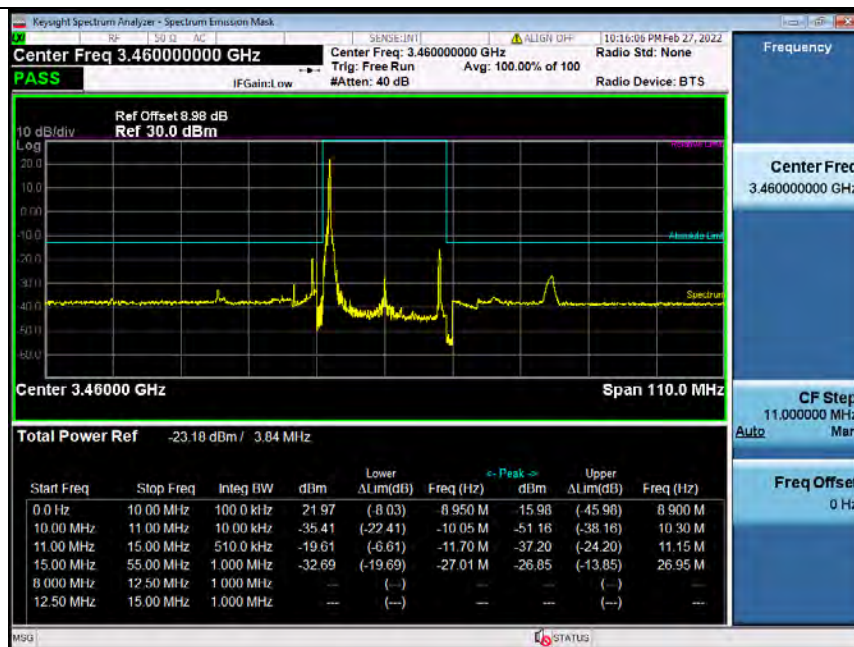
Band42H_20MHz_64QAM_LCH_3460MHz_RB_100_0_NTNV_Bandedge
