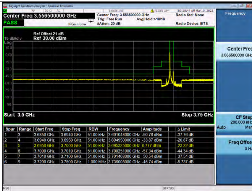
Band48_5MHz_16QAM_HCH_3697.5MHz_RB_1_0_NTNV (Integrated Power for 3693-3694MHz)
