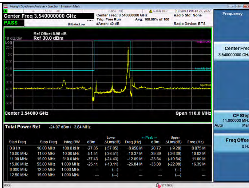
Band42H_20MHz_64QAM_HCH_3540MHz_RB_100_0_NTNV_Bandedge
