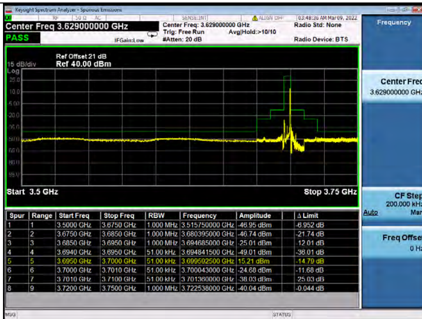
Band48_5MHz_QPSK_HCH_3697.5MHz_RB_1_24_NTNV (Integrated Power for 3701-3702MHz)
