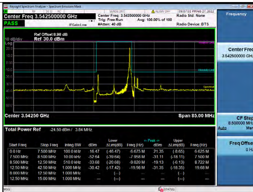
Band42H_15MHz_16QAM_HCH_3542.5MHz_RB_75_0_NTNV_Bandedge
