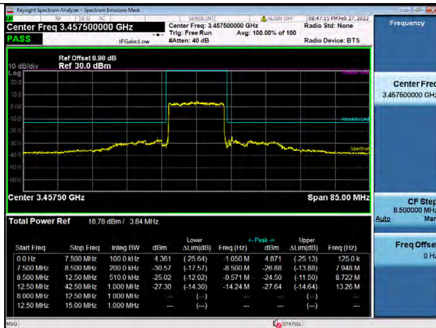
Band42H_15MHz_QPSK_LCH_3457.5MHz_RB_75_0_NTNV_Bandedge
