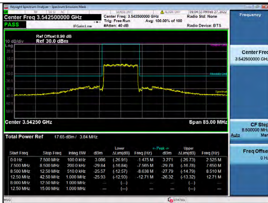
Band42H_15MHz_64QAM_HCH_3542.5MHz_RB_75_0_NTNV_Bandedge
