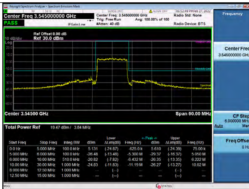
Band42H_10MHz_64QAM_HCH_3545MHz_RB_50_0_NTNV_Bandedge
