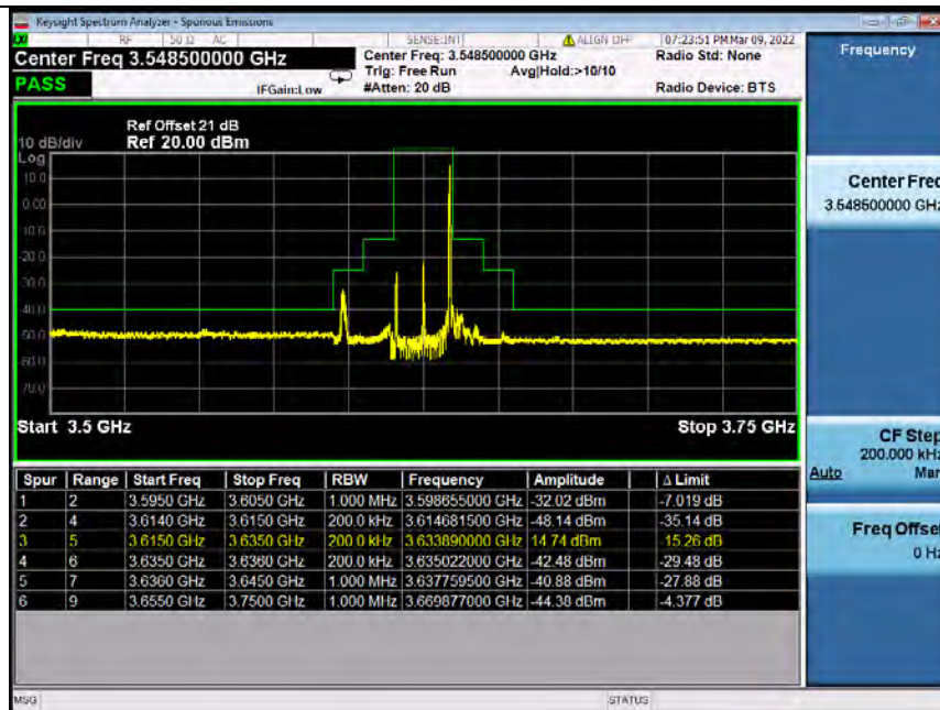
Band48_20MHz_64QAM MCH_3625MHz_RB_100_0_NTNV
