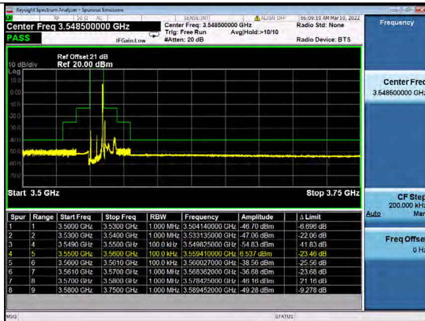
Band48_10MHz_64QAM_LCH_3555MHz_RB_50_0_NTNV
