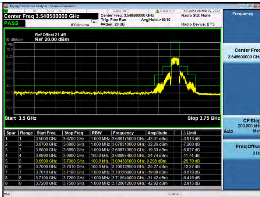
Band48_10MHz_64QAM_HCH_3695MHz_RB_50_0_NTNV
