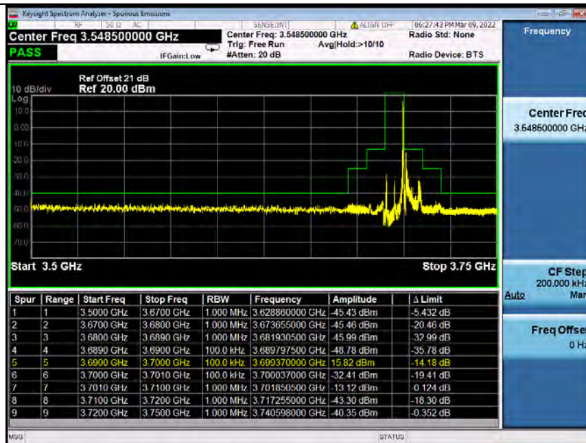
Band48_10MHz_64QAM_HCH_3695MHz_RB_50_0_NTNV
