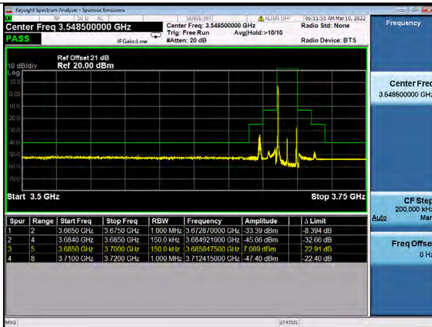
Band48_15MHz_64QAM_HCH_3692.5MHz_RB_1_74_NTNV
