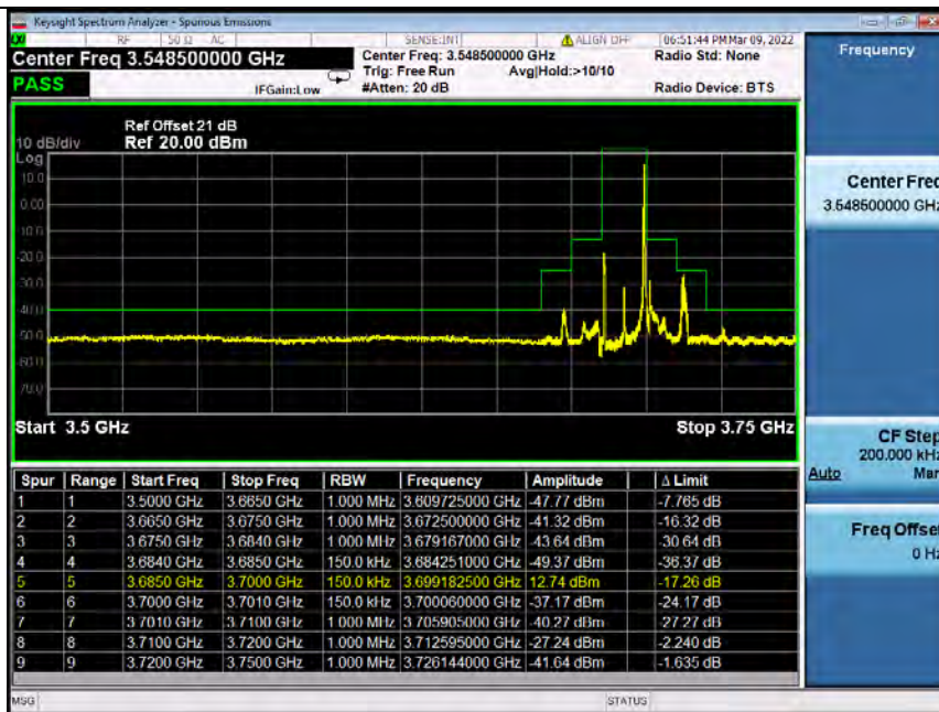
Band48_15MHz_16QAM_HCH_3692.5MHz_RB_75_0_NTNV
