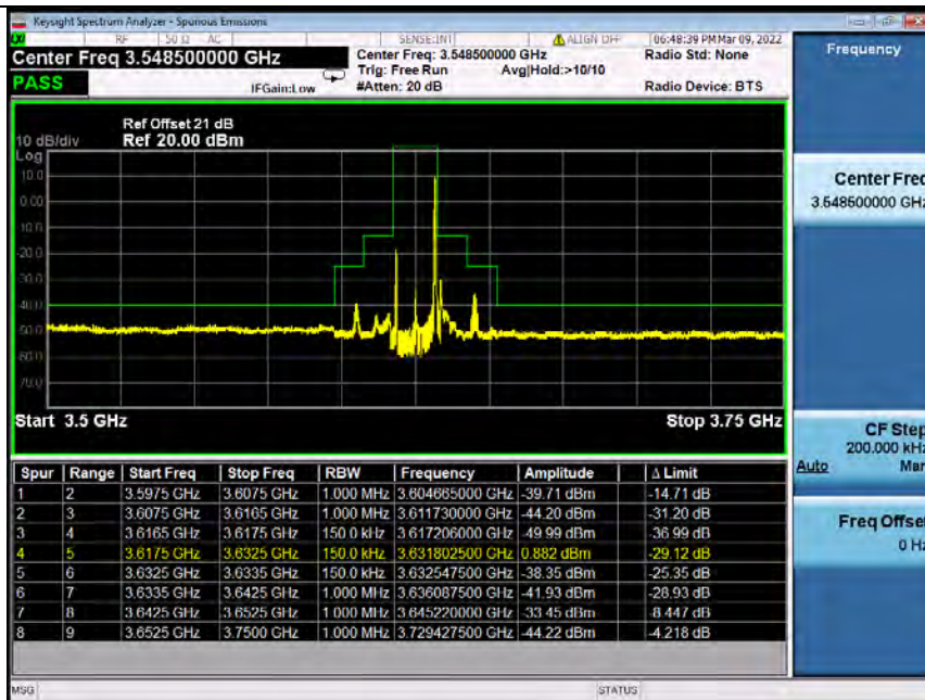
Band48_15MHz_16QAM MCH_3625MHz_RB_75_0_NTNV
