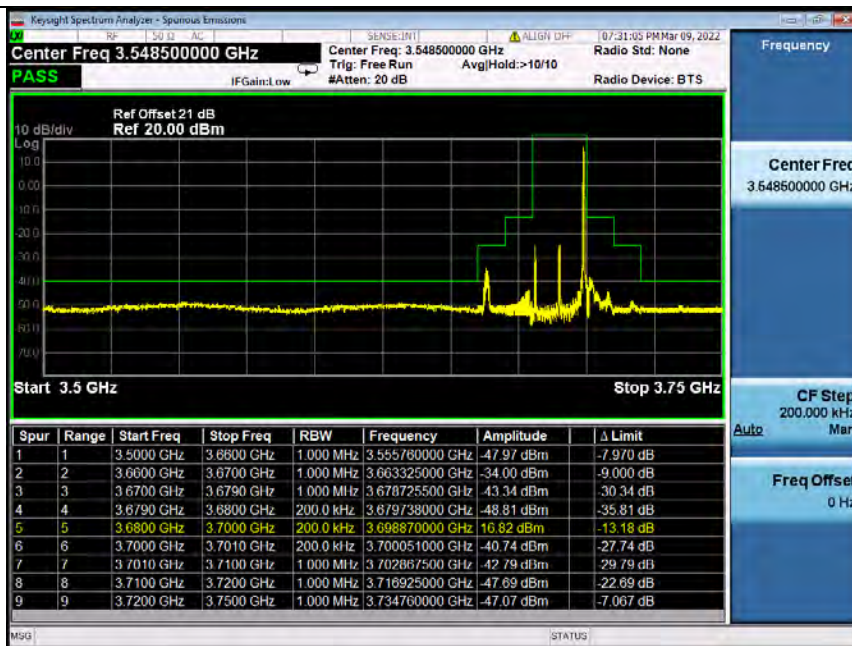
Band48_20MHz_64QAM_HCH_3690MHz_RB_100_0_NTNV
