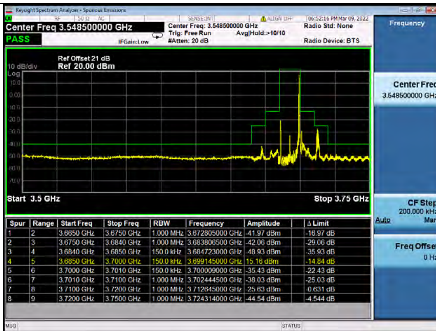
Band48_15MHz_64QAM_HCH_3692.5MHz_RB_75_0_NTNV
