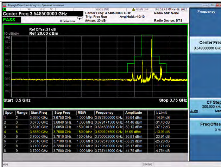
Band48_15MHz_QPSK_HCH_3692.5MHz_RB_75_0_NTNV
