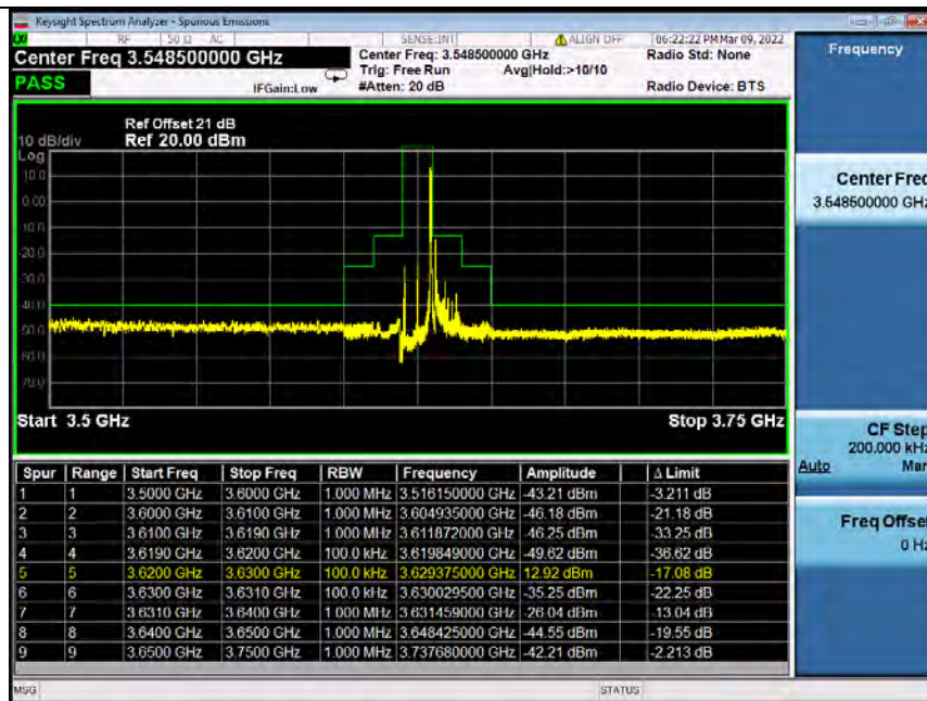
Band48_10MHz_64QAM MCH_3625MHz_RB_50_0_NTNV
