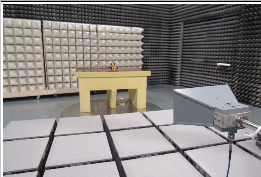
TEST SETUP BBHA9120D
