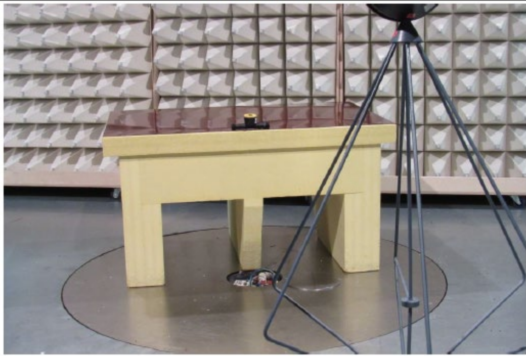
Radiated Setup 1
