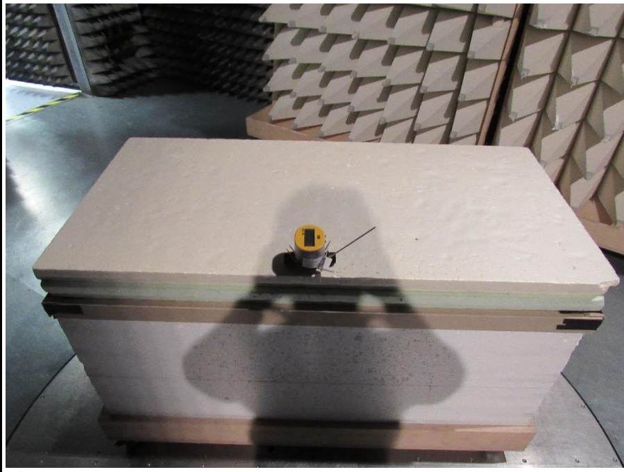
EUT Setup below 1GHz
