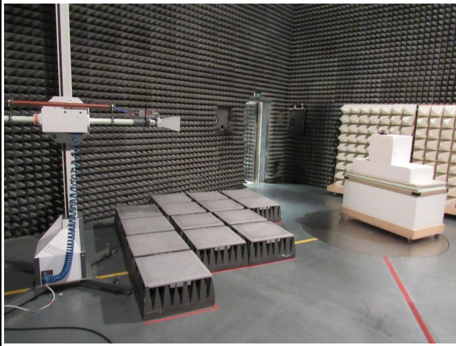
Test Setup above 1 GHz - II
