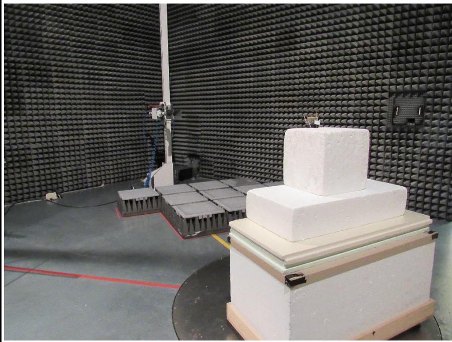
Test Setup above 1 GHz - I
