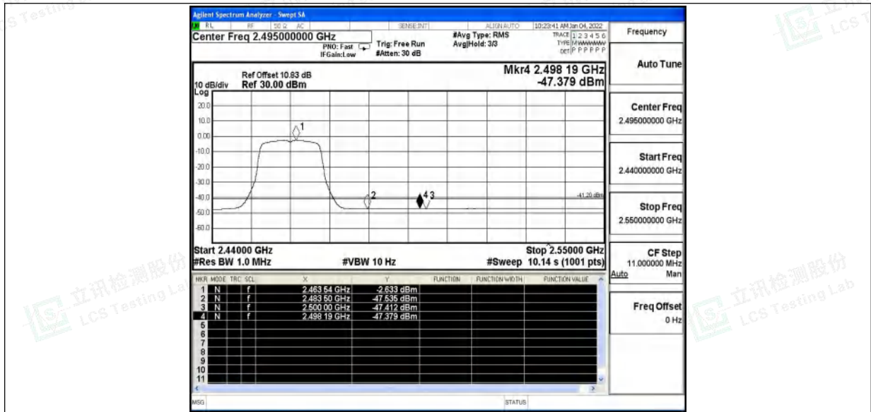
11G_Ant0_High_2462_Peak
