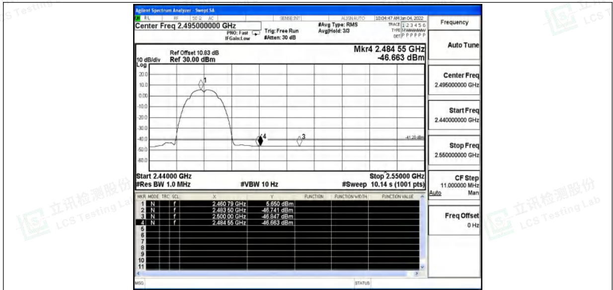
11B_Ant0_High_2462_Peak
