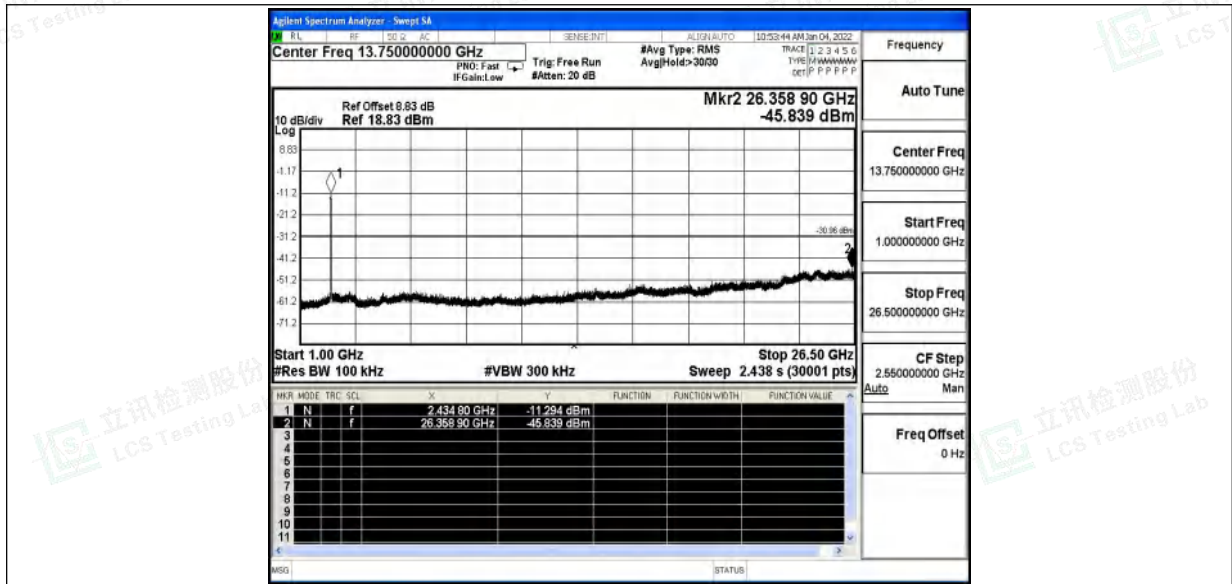
11N40SISO_Ant0_2452_0~Reference
