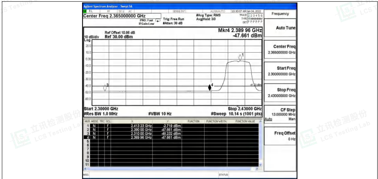
11N20SISO_Ant0_Low_2412_Peak
