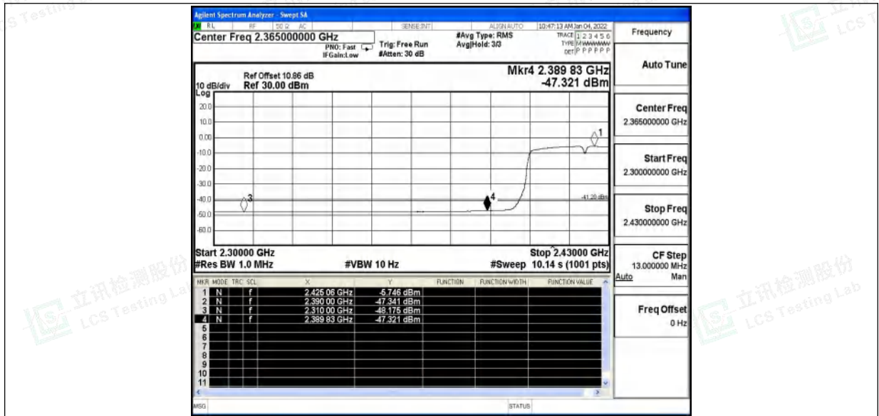
11N40SISO_Ant0_Low_2422_Peak
