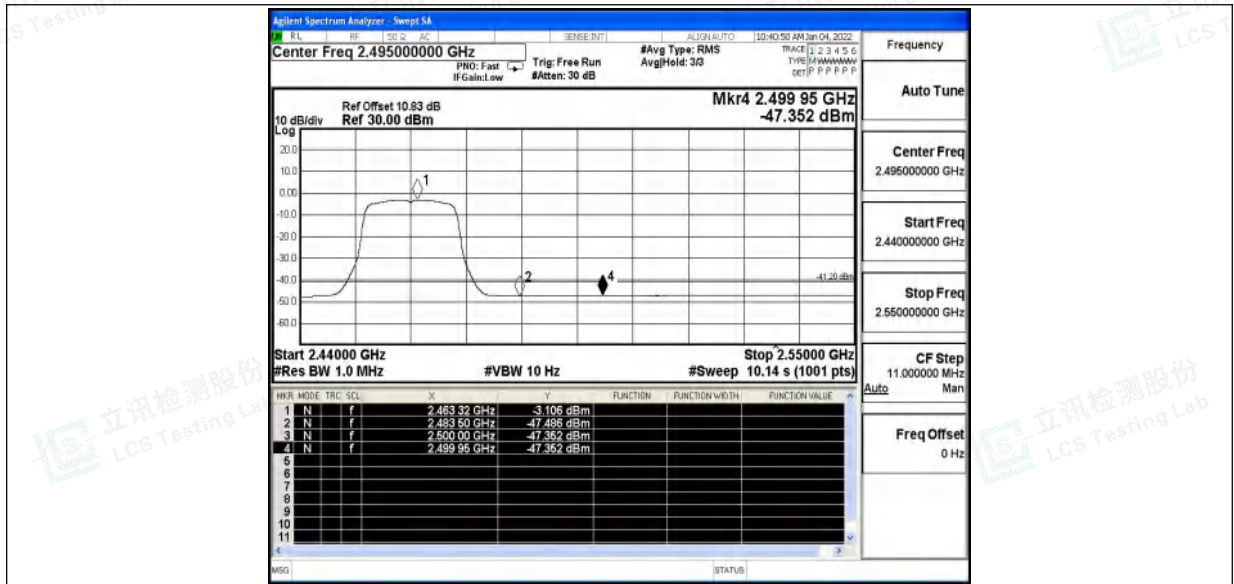
11N20SISO_Ant0_High_2462_Peak
