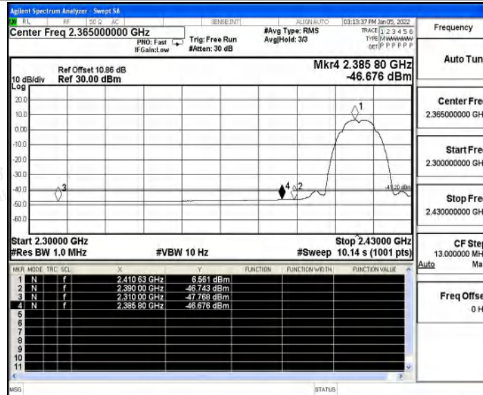
11B_Ant1_Low_2412_Peak
