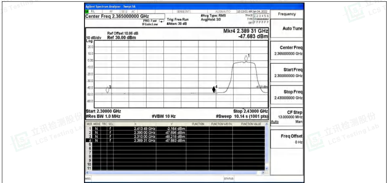
11G_Ant0_Low_2412_Peak
