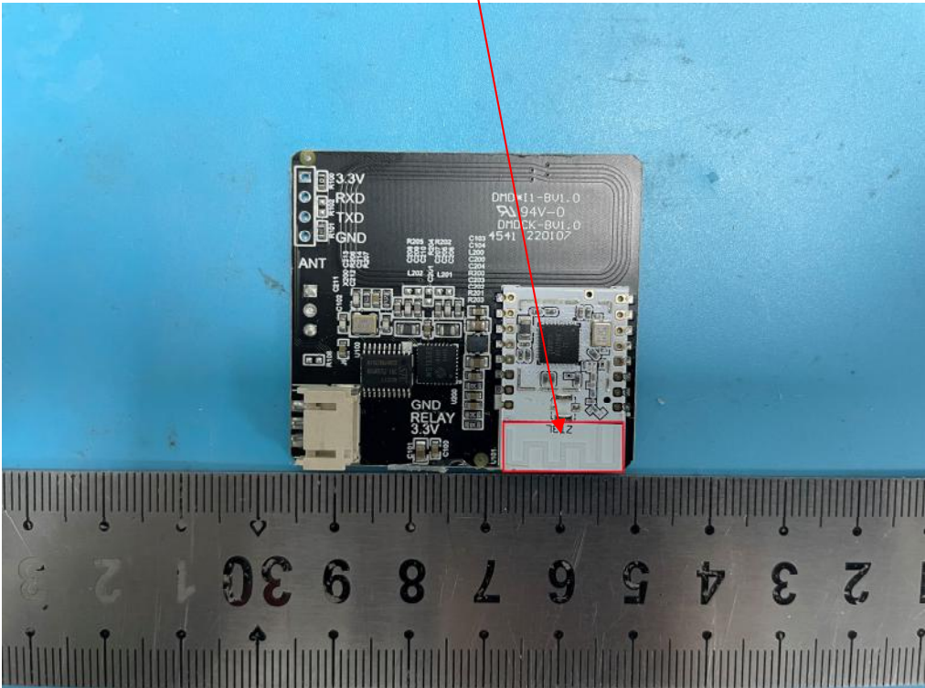
Zigbee Antenna
