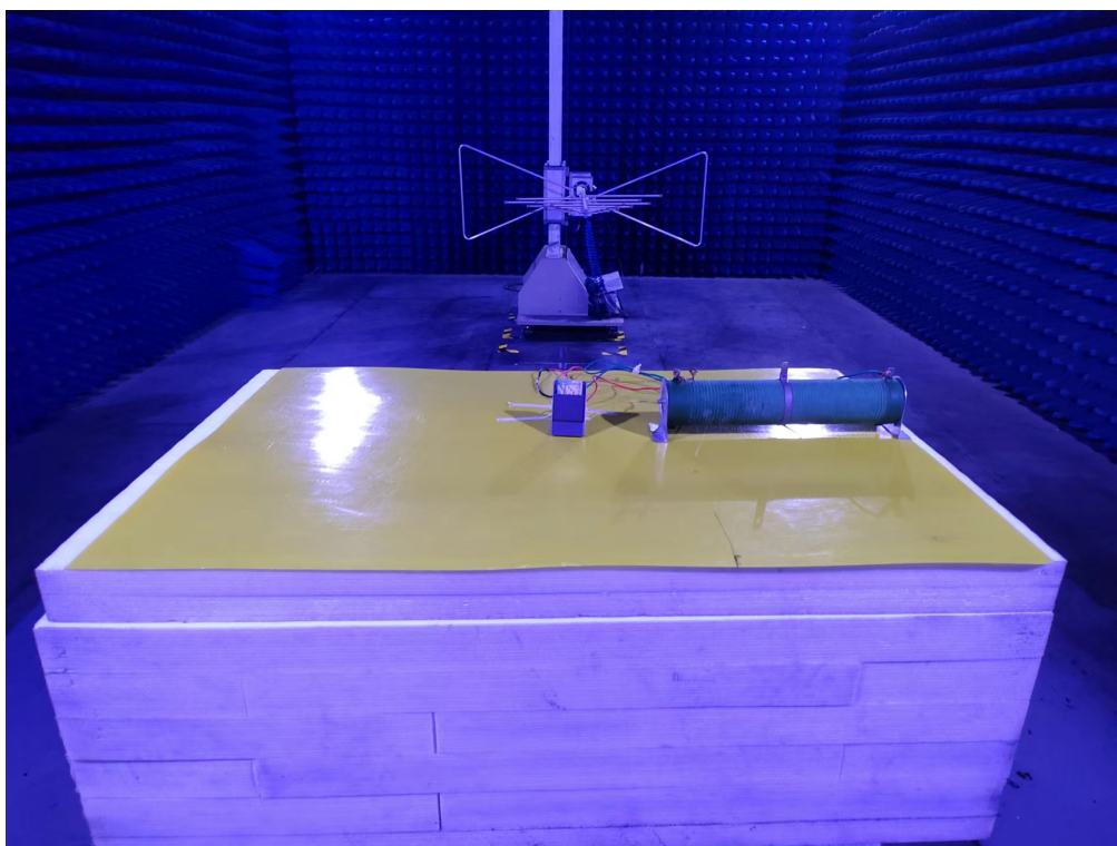
Photo of Radiated Emission Measurement (Above 30 MHz)
