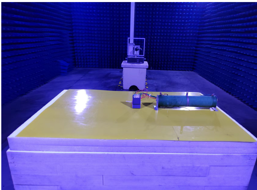
Photo of Radiated Emission Measurement (Below 30 MHz)
