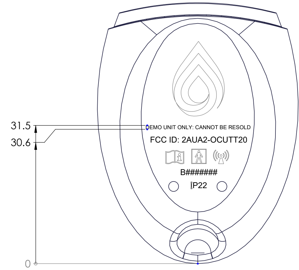
Scale 2:1 TrueTear 2.0 Demo Back Housing
