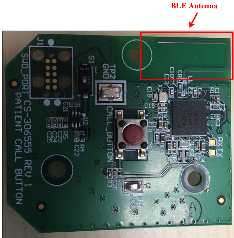
Photograph 3. BLE Antenna Location
