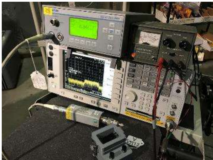
Bench Measurements including Power, PSD, Bandwidth
