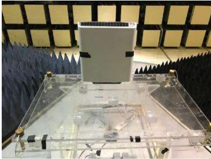
Radiated Emissions, Front, Below 1 GHz
