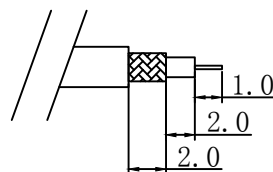
FPC STRIPPING DIM'S
