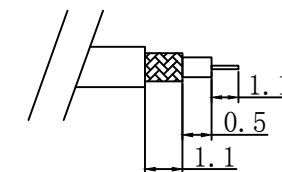
IPEX-4L STRIPPING DIM'S
