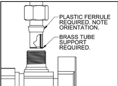
Figure 2: Supply Valve Connection
