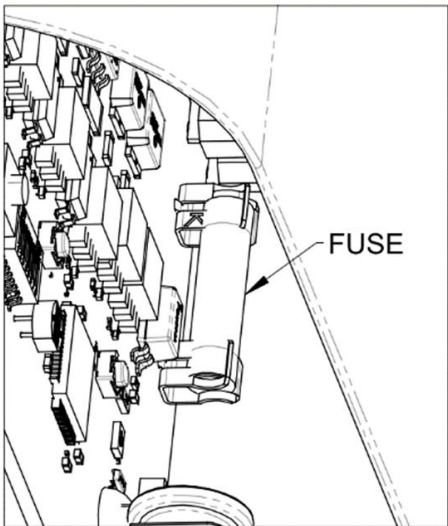
Figure 7: Fuse Replacement view from underside of bowl
