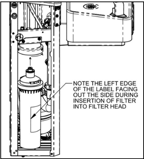
Figure 6: Filter Replacement
