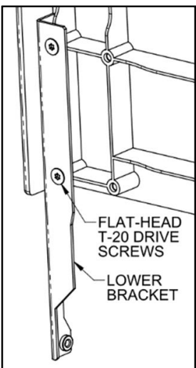
Figure 3: Bottle Filler Lower Brackets
