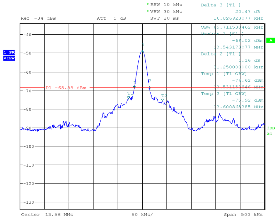
20-dB Channel Bandwidth & 99% Channel Bandwidth
