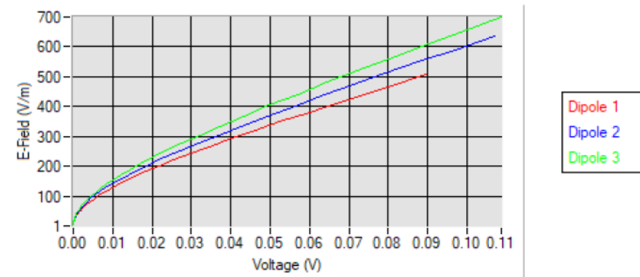
Calibration curves
