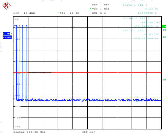
433.92MHz
