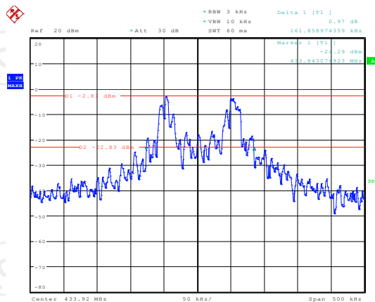
433.92MHz
