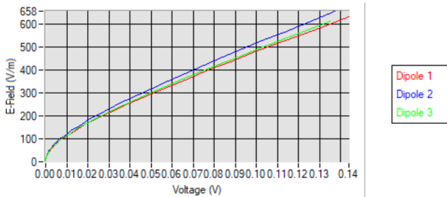
Calibration curves
