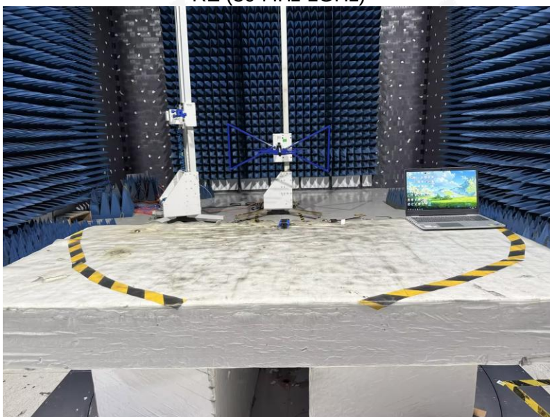
RE (30 MHz-1GHz)
