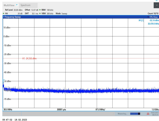
BLE_1M_Ant1_2440_30~1000
