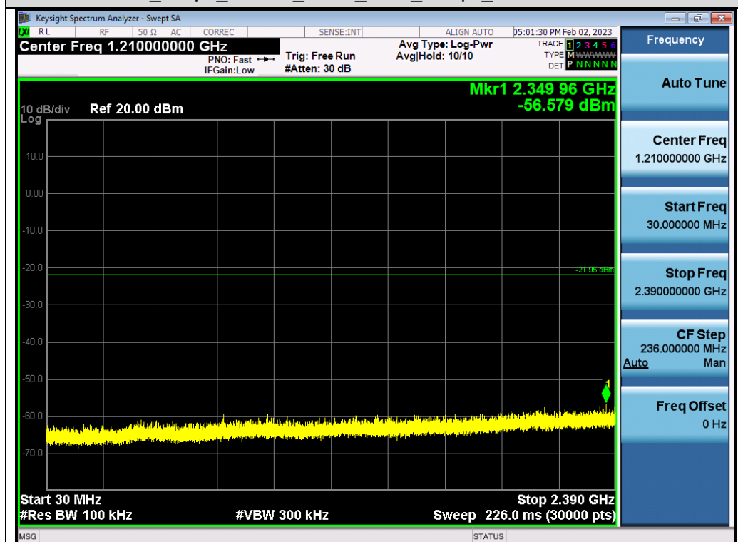
Test_Graph_BLE1M_ANT1_2402_1Mbps_Lower Band Emissions
