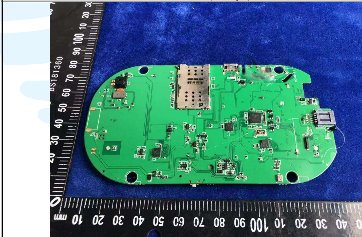
EUT Photo (Battery-2)
