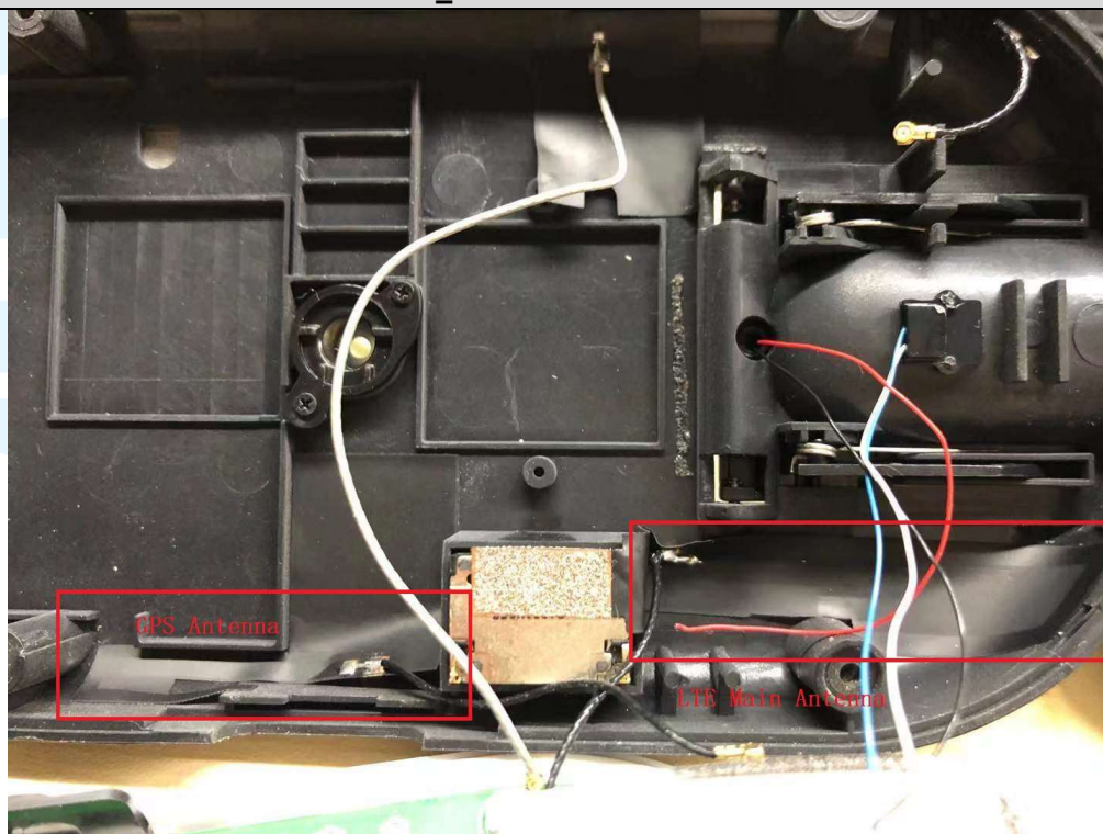
EUT Photo_GPS and LTE Main Antenna
