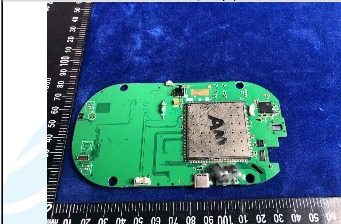
EUT Photo (Battery-2)
