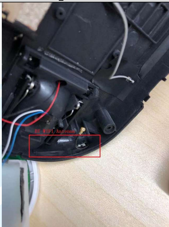
EUT Photo_BT & WIFI Main Antenna
