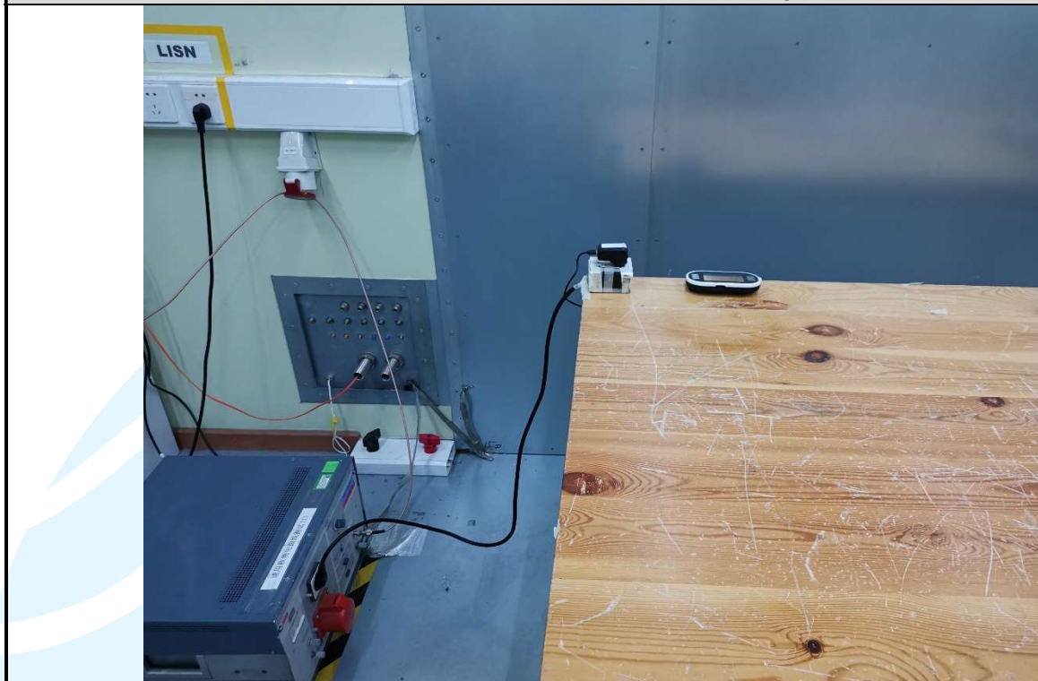
AC Conducted Emission Test Setup
