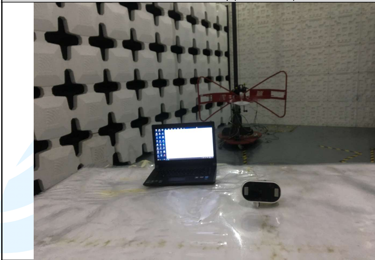
Radiated emission Test Setup (30 MHz~1 GHz)
