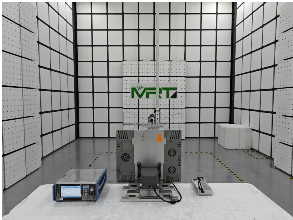
Description: Radiated Spurious Emission Test Setup for of 30MHz ~ 1GHz
