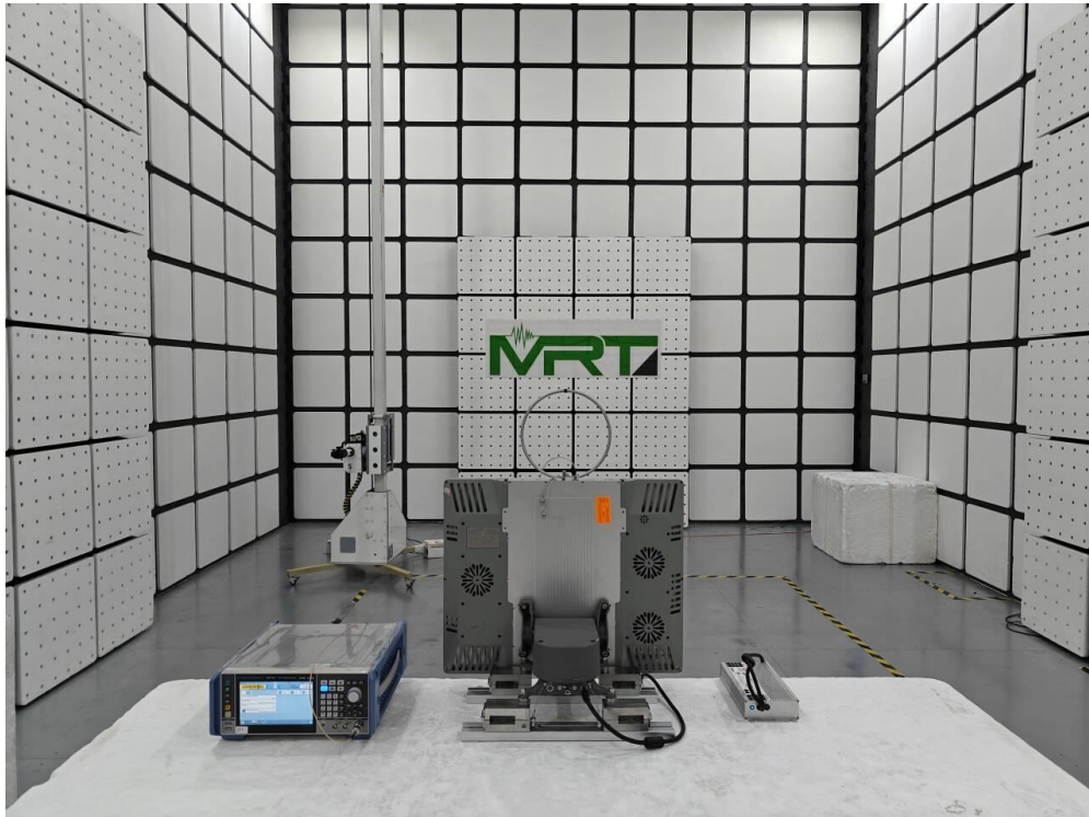
Description: Radiated Spurious Emission Test Setup of 9kHz ~ 30MHz
