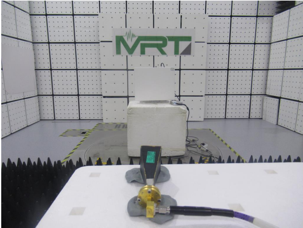
Description: Radiated Spurious Emission Test Setup of 50GHz ~ 75GHz
