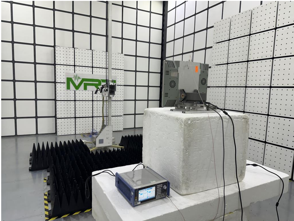
Description: Radiated Spurious Emission Test Setup of 18GHz ~ 40GHz
