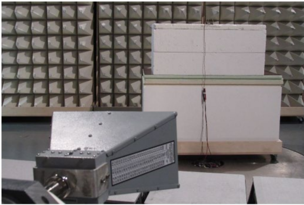
Radiated setup 1 GHz – 10 GHz
