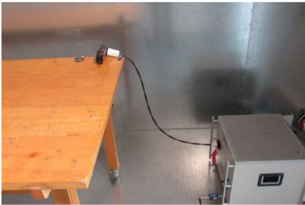
Conducted Setup
