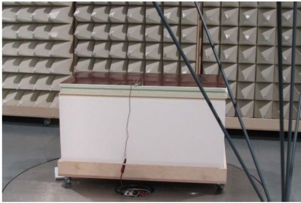
Radiated setup 30 MHz – 200 MHz
