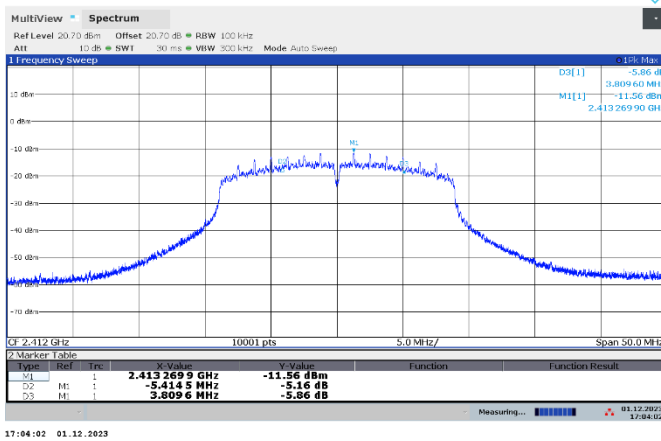
Figure 7.4-13: 6 dB bandwidth on 802.11n (MCS0) low channel
