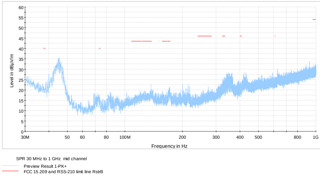
Figure 7.6-17: radiated spurious emissions from 30 MHz to 1000 MHz on 802.11b (11 Mbps) at mid channel
