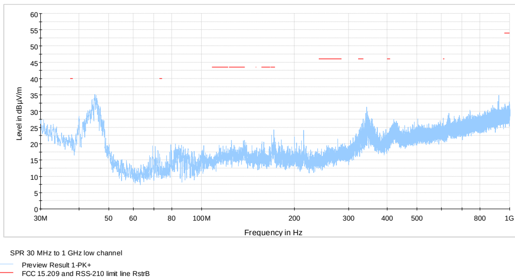
Figure 7.6-16: radiated spurious emissions from 30 MHz to 1000 MHz on 802.11b (11 Mbps) at low channel
