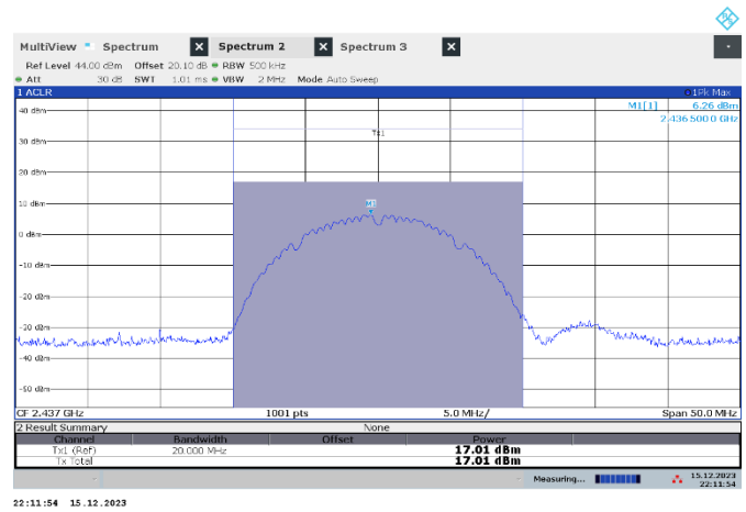
Figure 7.5-2: Output power on 802.11b (1 Mbps) mid channel
