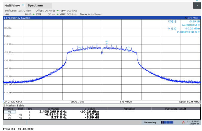
Figure 7.4-14: 6 dB bandwidth on 802.11n (MCS0) mid channel
