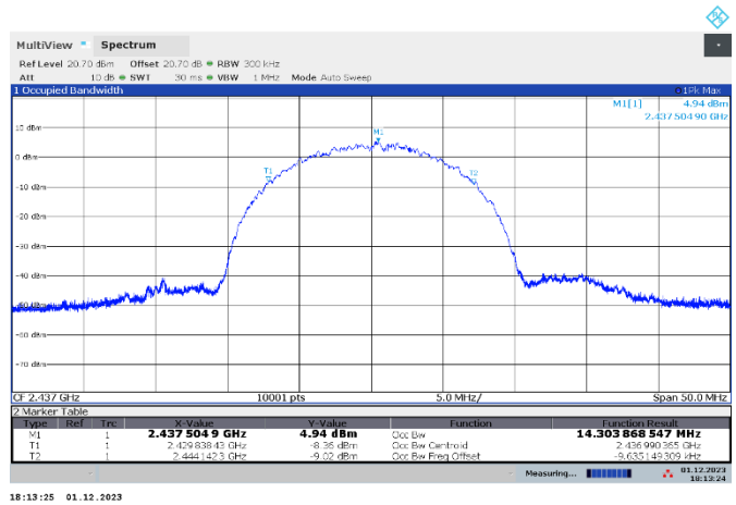
Figure 7.4-23: 99% occupied bandwidth 802.11b (11 Mbps) mid channel
