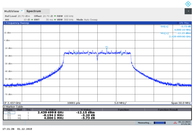
Figure 7.4-17: 6 dB bandwidth on 802.11n (MCS7) mid channel
