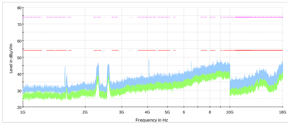
Figure 7.6-58: radiated spurious emissions from 1 GHz to 18 GHz on 802.11n (MCS0) at low channel
