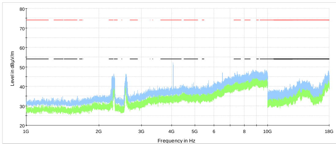
Figure 7.6-45: radiated spurious emissions from 1 GHz to 18 GHz on 802.11g (54 Mbps) at low channel
