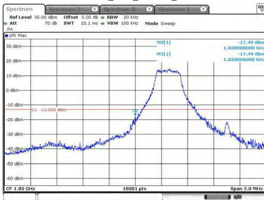
CH18607_1.4M_16-QAM_1RB0
