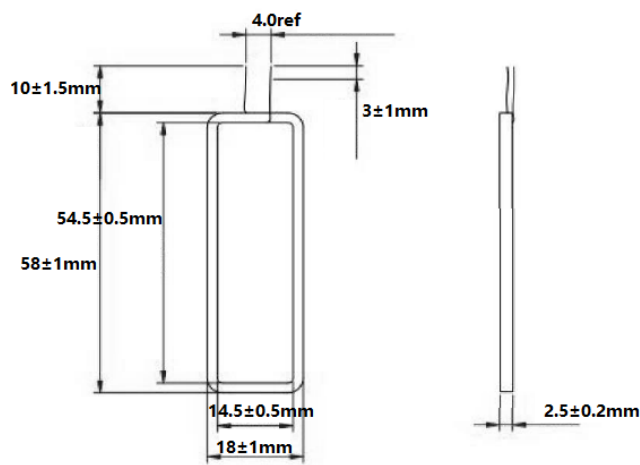
125KHz's antenna dimensions picture(Unit:mm)
