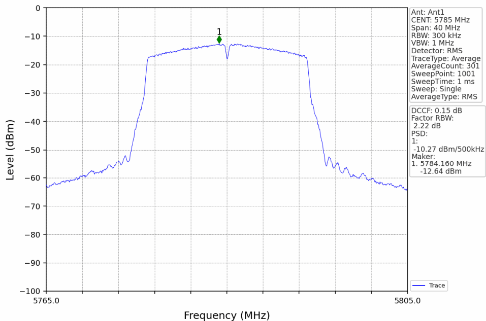
802.11ac(VHT20)_MCH_5785MHz_Ant1_NTNV
