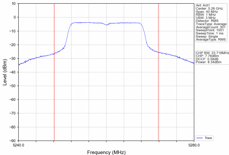
802.11a_LCH_5260MHz_Ant1_NTNV
