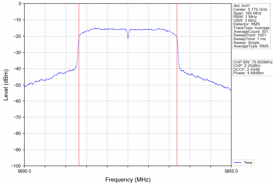
802.11ac(VHT80)_MCH_5775MHz_Ant1_NTNV
