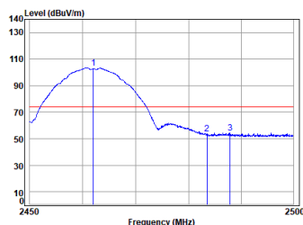
11b_TX_CH_11_Vertical-Peak
