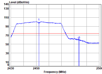
11n_HT(40M)_TX_CH_09_Vertical-Peak
