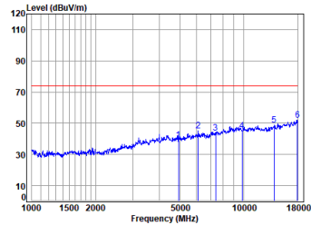
11b_TX_CH_11_Horizontal-Peak
