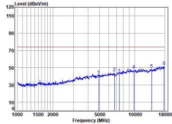
11b_TX_CH_11_Vertical-Peak
