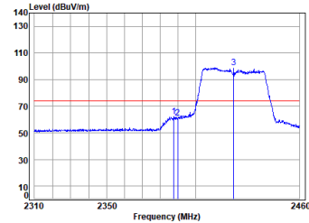
11n_HT(40M)_TX_CH_03_Vertical-Peak
