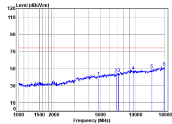
11n_HT(20M)_TX_CH_01_Horizontal-Peak
