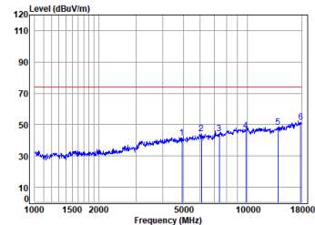
11n_HT(20M)_TX_CH_11_Vertical-Peak
