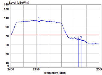
11n_HT(40M)_TX_CH_09_Horizontal-Peak
