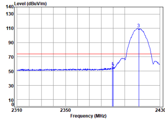
11b_TX_CH_01_Horizontal-Peak
