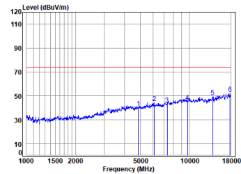
11n_HT(20M)_TX_CH_06_Horizontal-Peak
