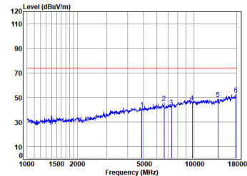
11n_HT(20M)_TX_CH_06_Vertical-Peak
