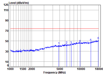
11b_TX_CH_06_Vertical-Peak
