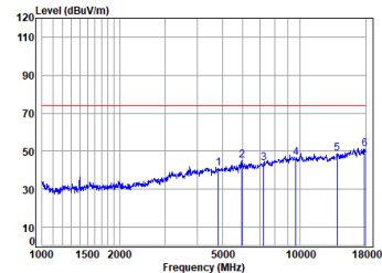
11n_HT(20M)_TX_CH_01_Vertical-Peak
