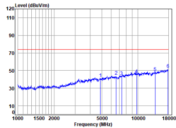
11b_TX_CH_06_Horizontal-Peak
