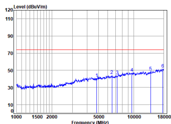
11b_TX_CH_01_Vertical-Peak
