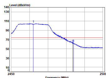
11n_HT(20M)_TX_CH_11_Vertical-Peak
