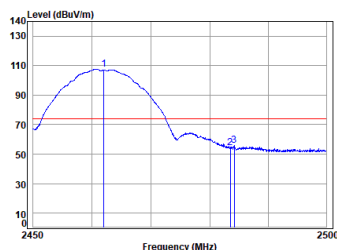
11b_TX_CH_11_Horizontal-Peak
