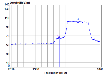
11n_HT(40M)_TX_CH_03_Horizontal-Peak
